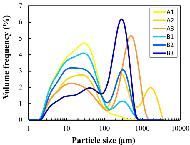
Fig. 2 Particle size distributions in the chocolate spreads
