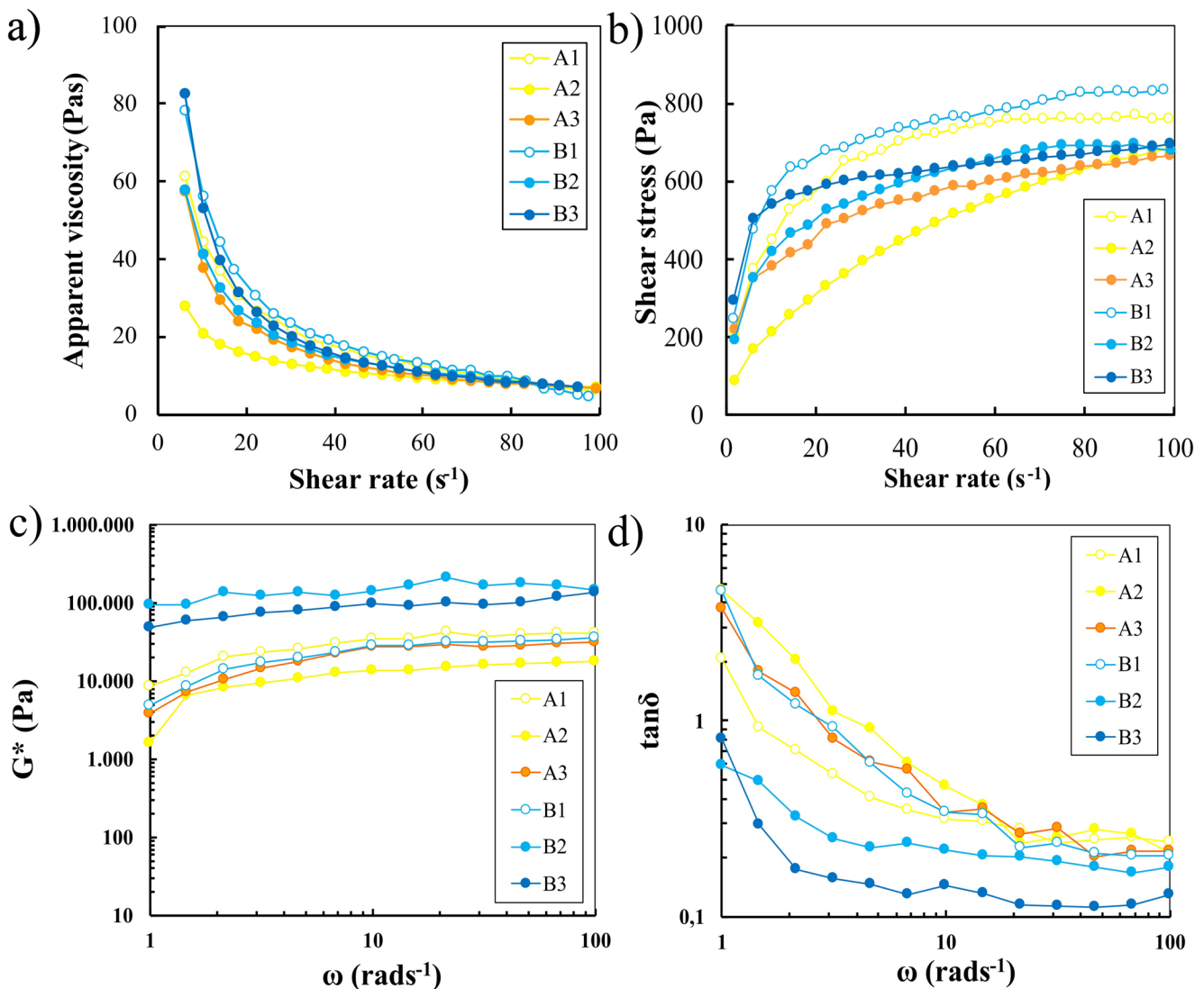
Fig. 3 Apparent viscosity–shear rate plots (a), flow curves (b) dependence of the complex modulus on frequency (c), and dependence of the loss tangent on frequency (d) of the chocolate spreads
