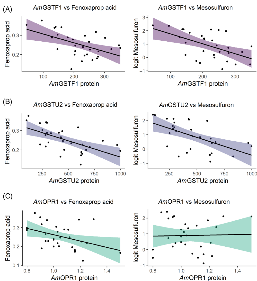
Figure 5. Fitted linear regression of three models with fenoxaprop metabolism (left) or mesosulfuron metabolism (right) predicted by protein expression of (A) AmGSTF1_{fenoxaprop} ( P < 0.01 ), AmGSTF1_{mesosulfuron} ( P < 0.01 ), (B) AmGSTU2_{fenoxaprop} ( P < 0.001 ), AmGSTU2_{mesosulfuron} ( P < 0.001 ) and (C) AmOPR1_{fenoxaprop} ( P < 0.05 ), AmOPR1_{mesosulfuron} ( P = 0.89 ). Solid lines show the fitted model with shaded regions showing 95% confidence limits and solid points are the original data used to fit the model.
