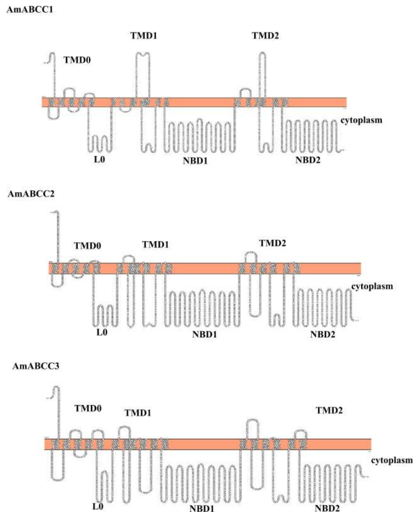
FIGURE 8 Predicted topology of AmABC sub-family C transporters. The topology models of AmABCC1, AmABCC2 and AmABCC3 membrane proteins illustrating the two cytoplasmic nucleotide-binding domains (NBDs) and the three transmembrane domains (TMDs).
