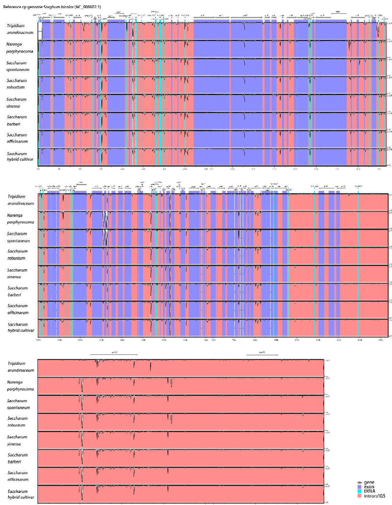
Figure 4. Chloroplast genomes were aligned using the mVISTA program with the annotation of S. bicolor as a reference. The X- and Y-scales indicate the coordinates within chloroplast genomes and the percentage of identity (50~100%), respectively. Gray arrows indicate the direction of transcription of each gene. Annotated genes are displayed along the top. The red block is the intron region, the pearlecent Aqua block is the tRNA region, and the purple block is the CDS region.
