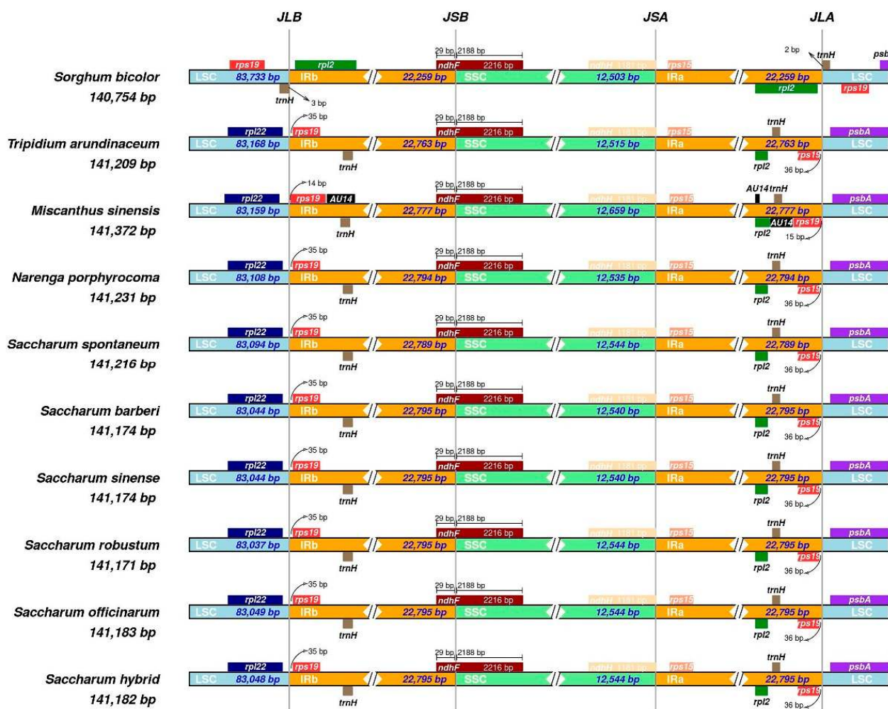
Figure 3. Comparison of border positions of LSC, SSC, and IR regions among nine Saccharinae species and S. bicolor . Genes are denoted by boxes, and the gap between the genes and the boundaries are indicated by the number of bases unless the gene coincides with the boundary. Extensions of genes are also indicated above the boxes.
