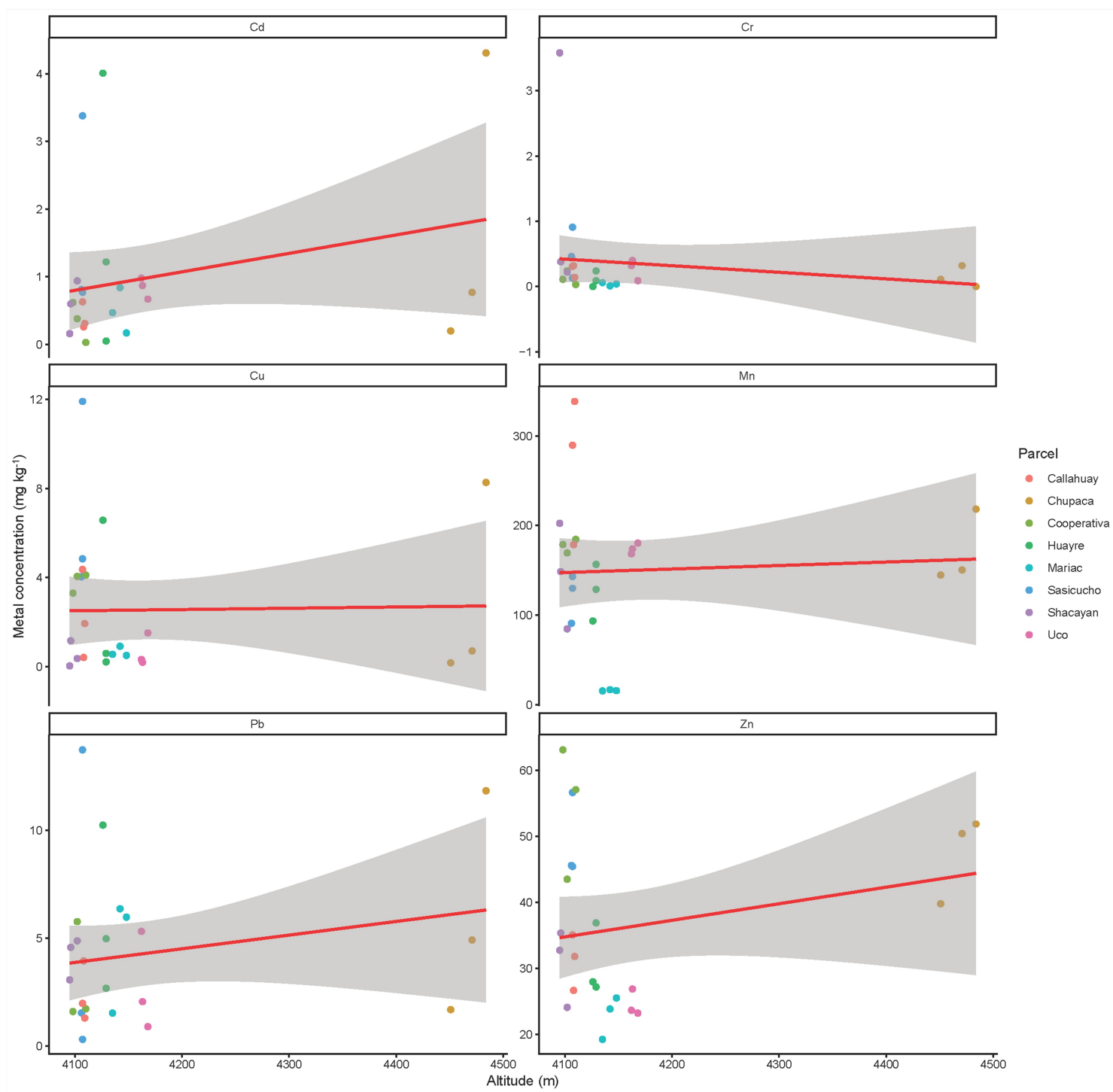
Figure 5 Relationship between altitude and trace metal concentrations in forage species across grazing plots in high-Andean ecosystems. Points represent individual samples colored by plot. Red lines indicate linear regression fits with 95% confidence intervals.
