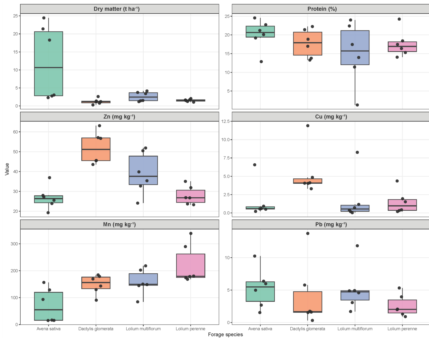
Figure 3 Variation in forage productivity, crude protein content, and selected trace metal concentrations among forage species. Boxplots represent the median and interquartile range, while points indicate individual observations.
