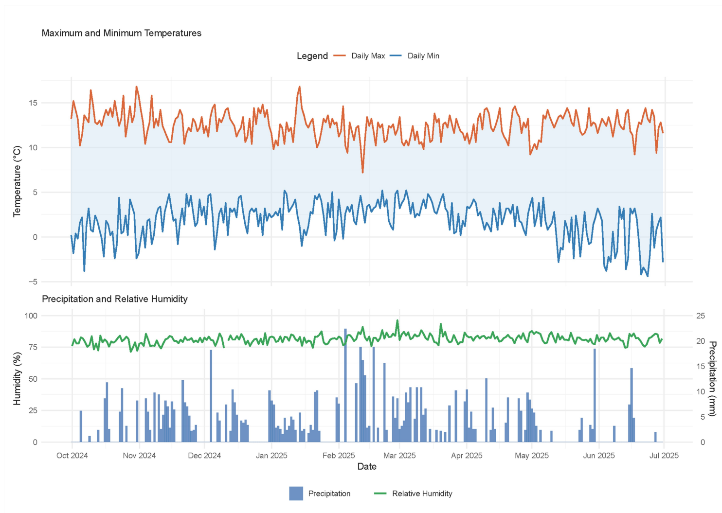
Figure 2 Temporal dynamics of temperature, precipitation, and relative humidity in high-Andean pastures during the study period.
