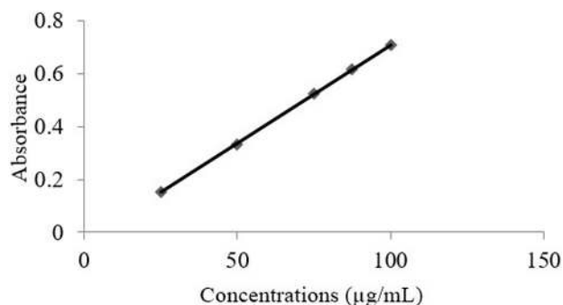
FIGURE 9 Relationship between concentration and absorbance of quercetin standards.
