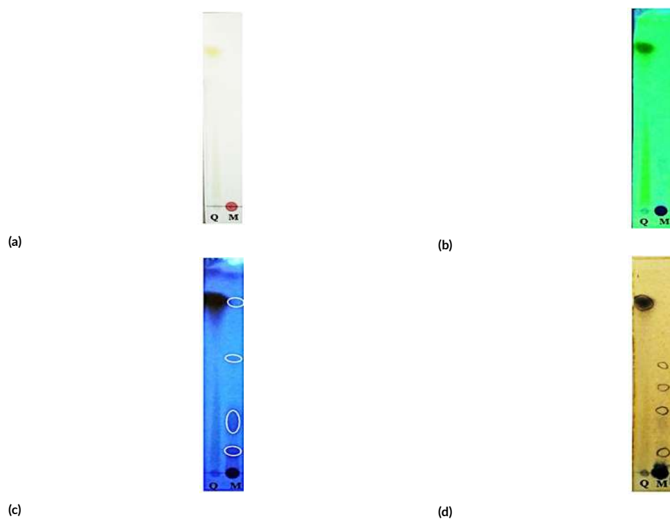
FIGURE 8 Standard TLC profile of quercetin (Q) and PME (M). Stationary phase: silica gel GF254; mobile phase: chloroform-acetone-formic acid (10:2:1). (a) Visible light. (b) UV254. (c) UV366. (d) 10% FeCl_3 spray reagent.
