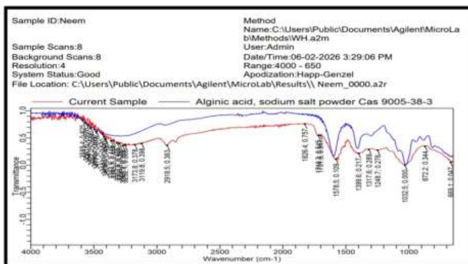
Figure 7: IR Spectrum of Azadirachta indica
