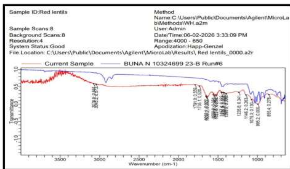
Figure 6 IR Spectrum of Lens culinaris
