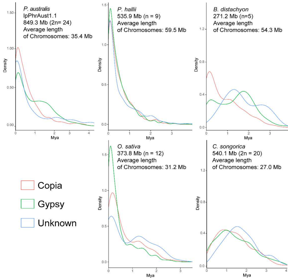
Figure S11. Distribution of insertion densities of different types of LTR-RTs in five Graminae plants. Including the P. australis (IpPhrAust1.1), Panicum hallii , Brachypodium distachyon , Oryza sativa , and Cleistogenes songorica .
