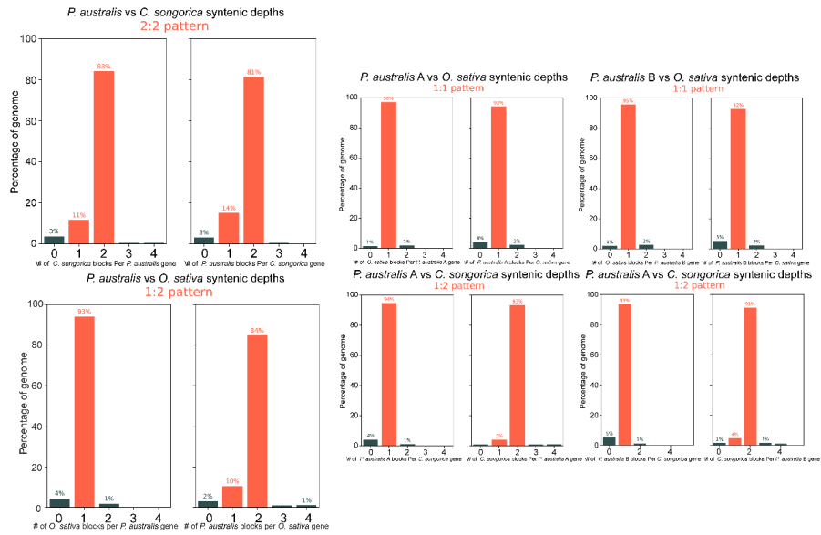
Figure S14. The syntenic depth of P. australis genomes/subgenomes with Cleistogenes songorica and O. sativa , respectively.
