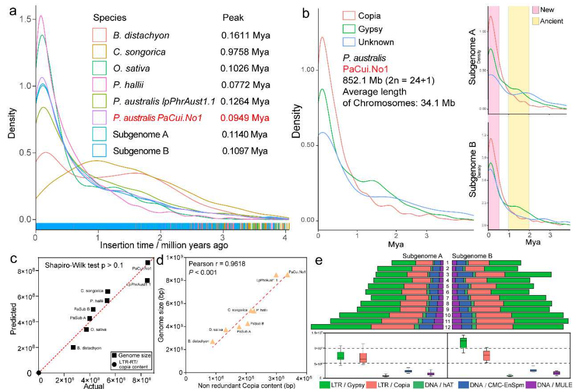
Fig. 3 Analysis of LTR-RTs in P. australis genomes. a Insertion times of LTR-RTs in eight genomes, including two P. australis subgenomes. b Insertion times of significant types of P. australis LTR-RTs. The right panel indicates the significant types of LTR-RT insertion times for subgenome A and subgenome B, respectively. c Normal QQ plot of Copia family content versus genome size for the P. australis genome. The normal distribution test using the Shapiro-Wilk (SW) method. d Pearson correlation analysis between Copia family content and genome size in the P. australis genome. e Differences in transposon content between two sets of subgenes in P. australis .
