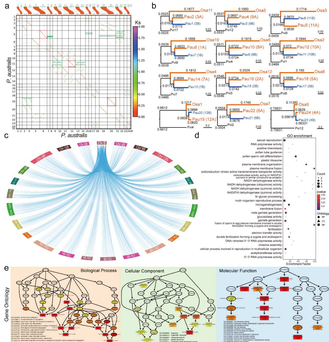
Fig. 2 Subgenomic isolation and B chromosome identification. a Dotplot of co-orthologs genes and Ks within P. australis genome. The color of the dot indicates the Ks of the gene pair. b Phylogenetic tree of genetic distances constructed based on single-copy homologous sequences. c Distribution of genes in the P. australis B chromosome in normal chromosomes. The blue connecting line in the figure indicates homology between the genes and those in the B chromosome with an E-value < 1e-10. d GO enrichment of genes expressed in the P. australis B chromosome. Genes with FPKM mean > 1 in chromosome B were retained for GO enrichment using clusterProfiler 2.0. e Directed acyclic map of GO enrichment of genes in the P. australis B chromosome. The more specific the molecular function, the lower the hierarchy. The ten most significant nodes are indicated by the boxes in the figure. The enrichment significance of each node is differentiated by color, from highest to lowest: red > orange > yellow.
