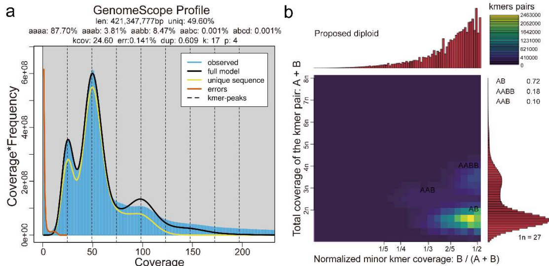
Figure S1. Survey analysis of the P. australis genome. a The 17-mer depth and number frequency distribution. Analyzed and visualized using GenomeScope 2.0. b Smudgeplot of the P. australis genome with relative coverage ( CovB / (CovA + CovB) ) in the horizontal, total coverage ( CovA + CovB ) in the vertical, and colors indicating the frequency of k-mer pairs. Each possible haplotype structure is presented as a "Smudge" on the graph, and the heat of the "Smudge" indicates the frequency of the haplotype structure in the genome.
