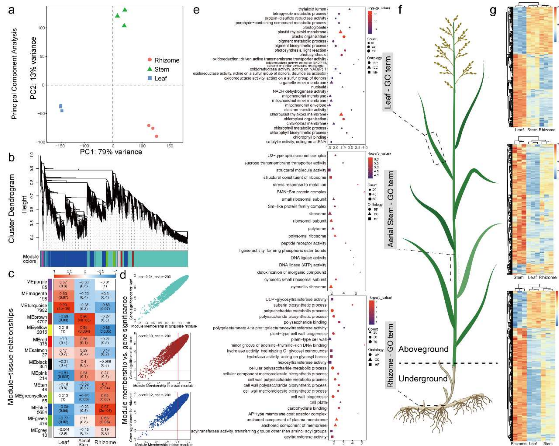
Fig. 5 Construction of the reed co-expression network. a Score scatter plots for the PCA model with nine samples. b Clustering dendrogram of gene based on the topological overlay. WGCNA analysis was performed after screening based on gene expression FPKM mean > 1. Each branch of the gene dendrogram corresponds to one module; different colors represent different modules. c Heatmap of gene co-expression network module-tissue association. Each row corresponds to a module characteristic gene (eigengene), and each column corresponds to a specific tissue. Each cell contains the corresponding correlation value and P-value, and indicates the strength of the correlation according to the color. d A scatterplot of Gene Significance (GS) for weight vs. Module Membership (MM) in three module eigengene. There is a highly significant correlation between GS and MM in this module, illustrating that genes highly significantly associated with a trait are often also the most critical elements of modules associated with the trait. The red lines indicate the thresholds for |MM| > 0.8 and |GS| > 0.2 , respectively. e Bubble diagram showing the results of GO enrichment of genes contained in the module eigengene. f Pattern map of reed plants (Created by Biorender, https://www.biorender.com ). g The heatmap shows the changes in FPKM based on log2 in the module eigengene.
