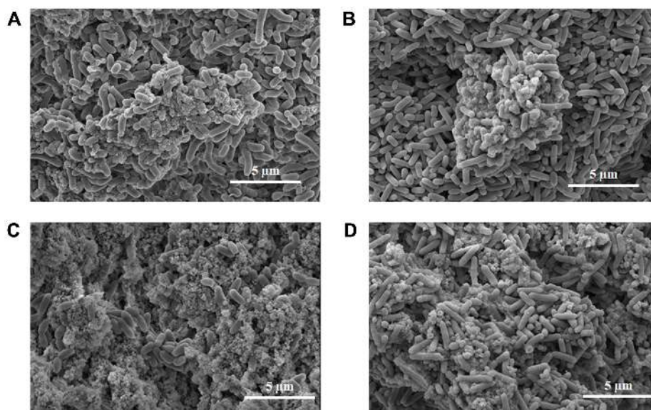
Fig. 4. Field-emission scanning electron microscopy (FE-SEM) of strain AK13 in B4 medium and B4L medium.
