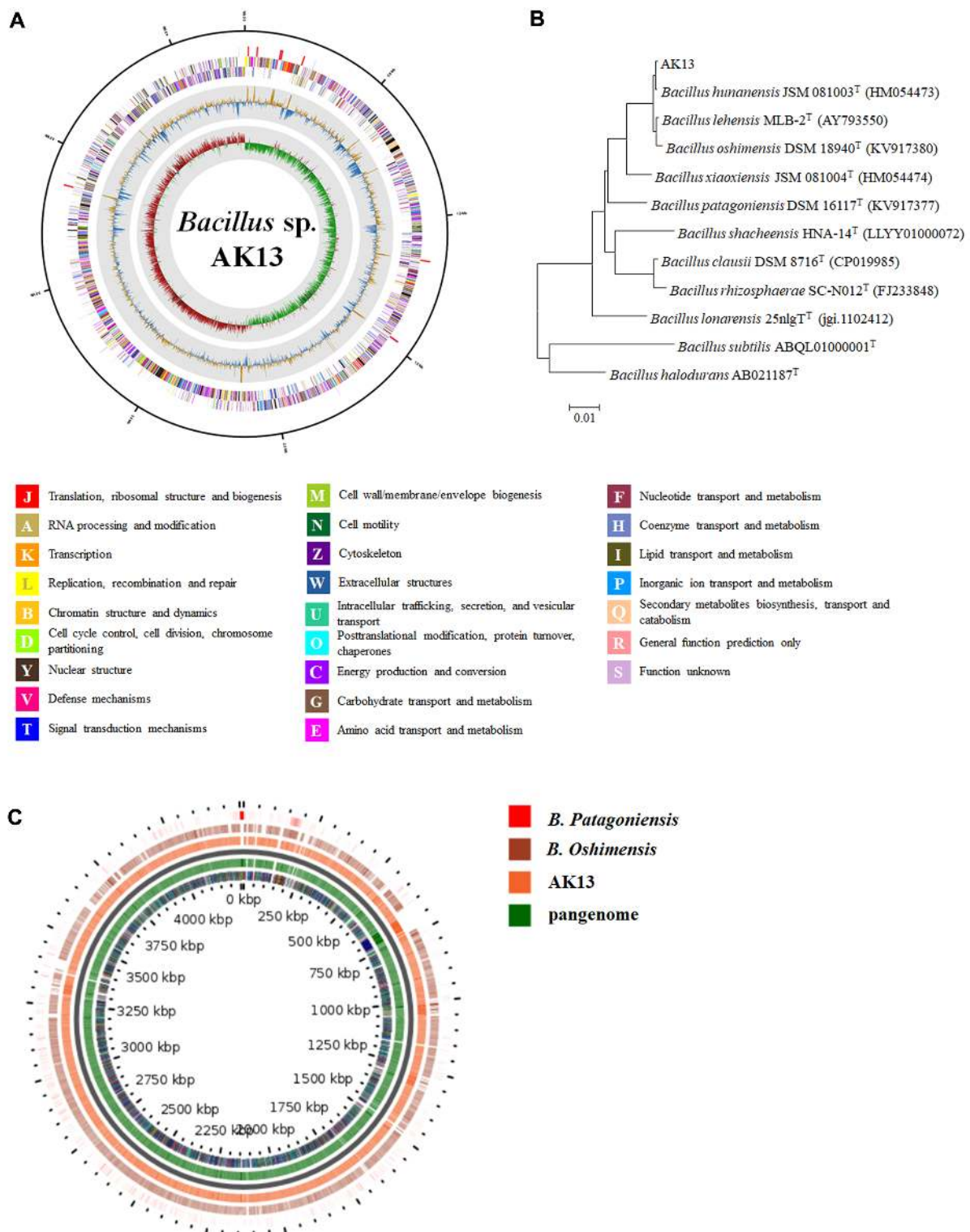
Fig. 1. Whole-genome sequencing and genome comparison analysis between AK13 and other alkaliphilic Bacillus .
