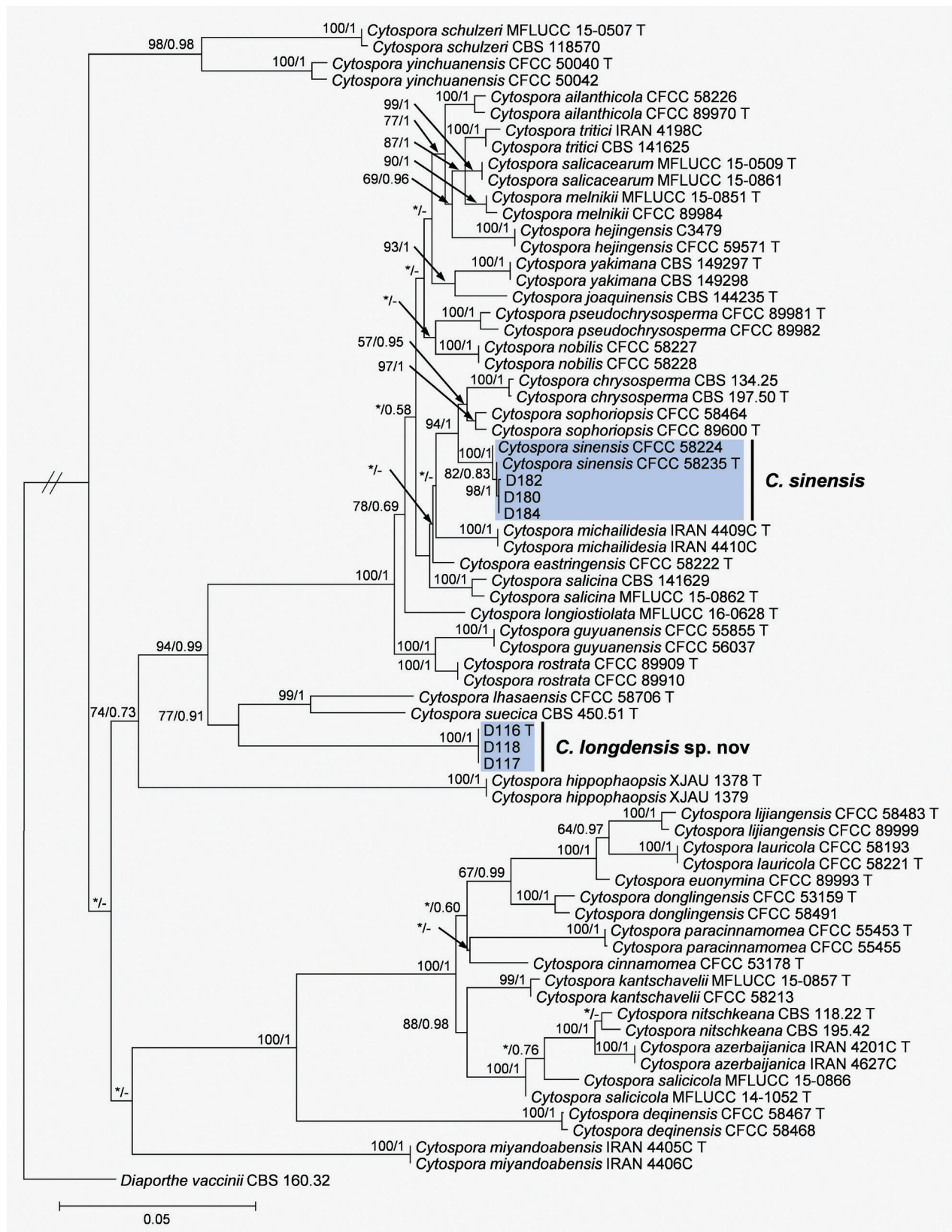
Figure 1. Phylogenetic tree of Cytospora based on maximum likelihood analysis of a combined DNA sequence dataset of ITS, act , rpb2 , tef1-a , and tub2 genes. Bootstrap values \geq 50\% (maximum likelihood) and posterior probabilities \geq 0.5 (Bayesian) are presented at the branches. Values lower than these thresholds are marked with “*”, and absent are marked with “-”. Type materials are marked with “T”. Isolates from this study are highlighted in blue. The tree was rooted to Diaporthe vaccinii (CBS 160.32).
