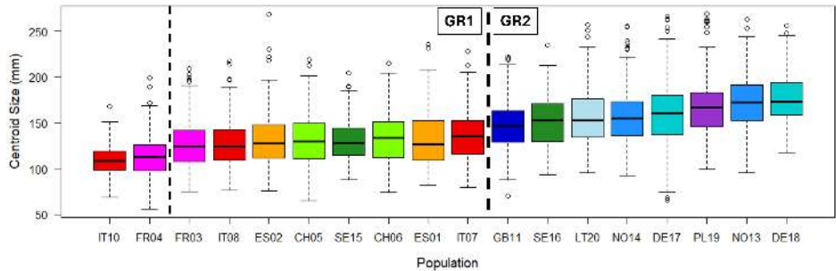
Figure 7. Boxplots showing the variation in centroid size values (mm) for the 419 trees belonging to the 18 populations analyzed. Boxes represent the interquartile range (IQR, 25th to 75th percentiles), the bold black line inside each box is the median, and the whiskers cover \pm 1.5 \times IQR. Circles indicate outliers. Populations are sorted by increasing the mean value of the centroid size. The dotted line separates populations belonging to the group 1 (GR1) and group 2 (GR2). The same color code of Figure 4 is used.
