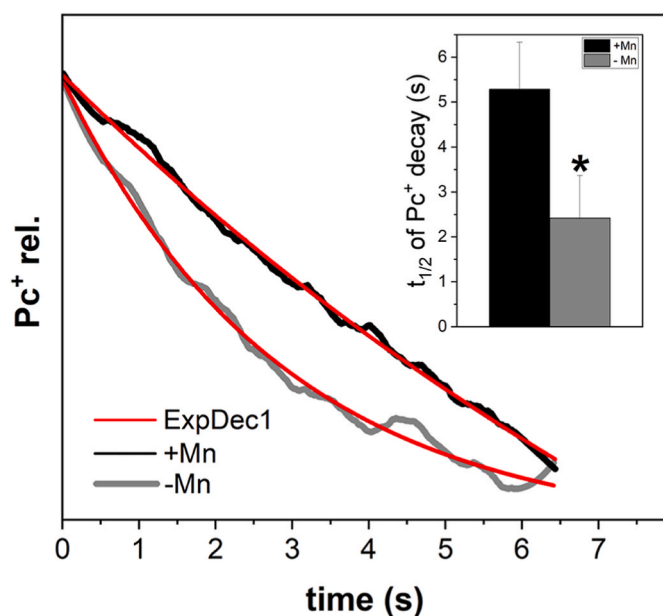
Fig. 6. Re-reduction kinetics of Pc + after FR illumination. The kinetics of Pc + re-reduction in Marchantia thalli indicated as black and grey for + Mn and -Mn, respectively, were monitored in the dark, after 5s exposure to FR light. Decay signals for P700 + were fitted with single exponential function (red traces). The curves represent an average of 6 measurements for each sample. The inset show the half times ( t_{1/2} ) calculated for Pc + decay (samples from three independent cultures, n = 6 ). Statistical significance (* P < 0.05 ) was assessed by Student's t -test.
