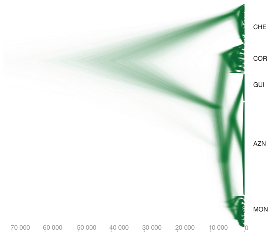
FIG. 5. Densitree of the Carex helodes individuals analysed. 95% CI (confidence interval) phylogenetic trees from BEASTvntnr analysis are shown in green. The x-axis gives the time in years. Population names are indicated.
