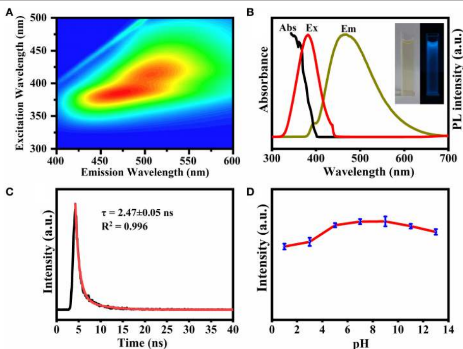
FIGURE 4 | (A) Excitation-emission matrix for UV-vis absorption spectra of CQDs. (B) UV-vis absorption, PL excitation and emission spectra of the CQDs. Inset shows images of the CQDs under daylight (left) and UV irradiation (right). (C) Time-resolved PL decay for the CQDs. (D) Effect of pH on the fluorescence stability of CQDs. For the luminescence spectra, the excitation wavelength was kept at 360 nm.
