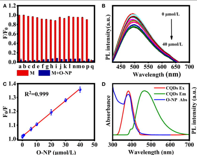
FIGURE 5 | (A) Luminescence quenching of CQDs by single compound M (100 \mu\text{mol/L} , red) and in mixed solutions of M with 100 \mu\text{mol/L} O-NP (blue). a, blank; b, \text{K}^+ ; c, \text{Pb}^{2+} ; d, \text{Ba}^{2+} ; e, \text{Ca}^{2+} ; f, \text{Hg}^{2+} ; g, \text{Na}^+ ; h, \text{Zn}^{2+} ; i, \text{Mg}^{2+} ; j, \text{Cr}^{3+} ; k, \text{Cu}^{2+} ; l, 3-NT; m, 3-NP; n, DNT; o, 2,4,6-TCP; p, NB; q, O-NP. (B) Fluorescence spectra of CQDs in the presence of O-NP at 0–40 \mu\text{mol/L} (excitation: 360 nm). (C) Dependence of F_0/F on the concentration of O-NP. (D) The absorption spectrum of O-NP, PL excitation, and emission spectra of CQDs.
