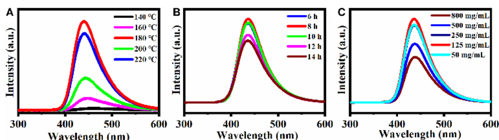
FIGURE 1 | Effect of different conditions on the fluorescence spectra: (A) Synthesis temperature, (B) Synthesis reaction time, and (C) Concentration of CQDs in solution. Excitation wavelength: 360 nm.
