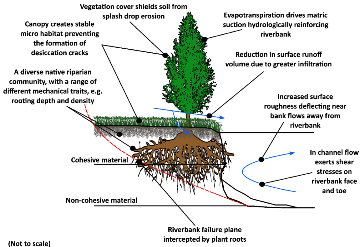
FIGURE 1 | Diagram depicting the influence of vegetation on riverbank erosion. [Color figure can be viewed at wileyonlinelibrary.com ]
