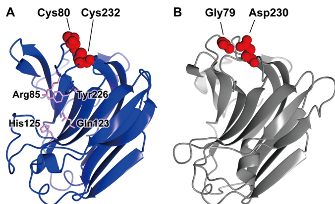
FIGURE 8. Homology modeling of NitAly and PyAly. The structures of NitAly (A, residues 34–242) and PyAly (B, residues 13–216) were predicted using the PHYRE2 program (63) and P. aeruginosa alginate lyase PA1167 (Protein Data Bank code 1vav) as the template (15) with 100% confidence, respectively. A, Cys-80 and Cys-232 are shown by red globules. The residues Arg-85, Gln-123, His-125, and Tyr-226, which correspond to the suggested catalytic residues in PA1167 (15, 21), are shown by pink sticks. B, Gly-79 and Asp-230 are shown by red globules.
