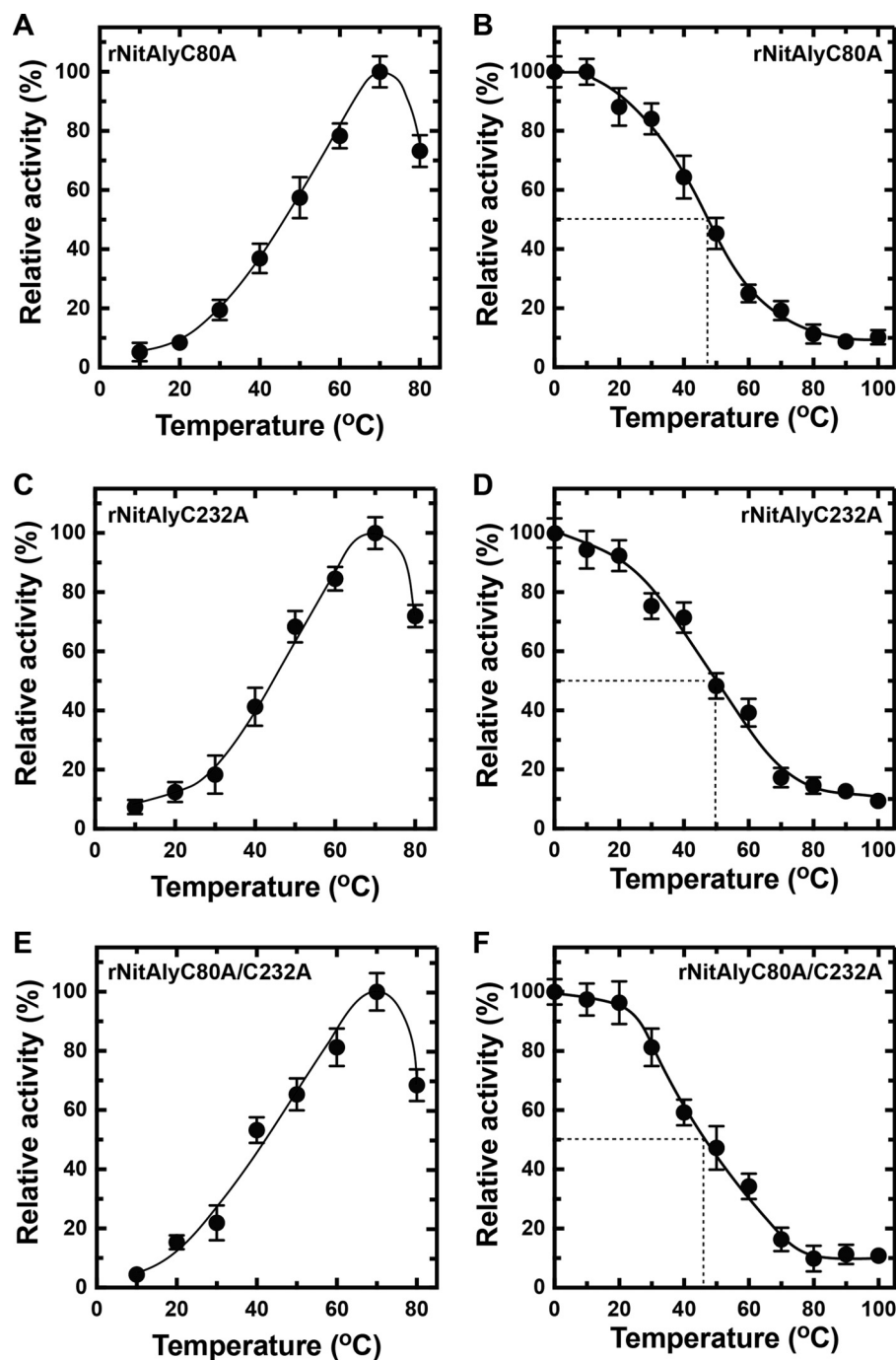
FIGURE 9. Effects of cysteine residue mutations in rNitAly on temperature dependence and heat stability. A, C, and E, temperature dependence of alginate lyase activity of rNitAlyC80A (A), rNitAlyC232A (C), and rNitAlyC80A/C232A (E). Assays were performed as described for Fig. 5A. Relative activities at 100% were equivalent to 1,520 units/mg (A), 1,630 units/mg (C), and 1,480 units/mg (E). B, D, and F, heat stability of rNitAlyC80A (B), rNitAlyC232A (D), and rNitAlyC80A/C232A (F). Assays were performed as described for Fig. 6A. Relative activity at 100% was equivalent to 970 units/mg (B), 1,060 units/mg (D), and 960 units/mg (F). All assays were repeated three times, and the data are shown as mean \pm S.D.
