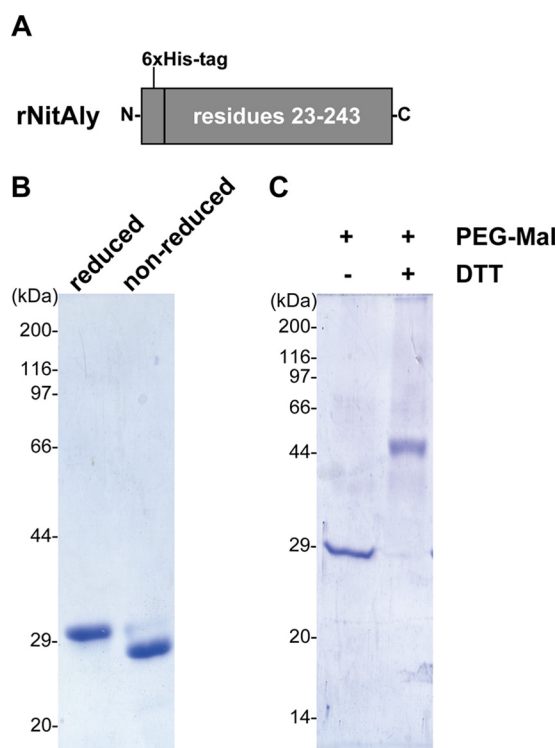
FIGURE 2. Bacterial expression and purification of rNitAly. A, schematic drawing of rNitAly. B, SDS-PAGE of purified rNitAly. Reduced and non-reduced indicate that the samples were prepared in the presence and absence of 20 mM DTT, respectively. C, SDS-PAGE of PEG-Mal-labeled rNitAly pretreated in the presence and absence of 20 mM DTT.
