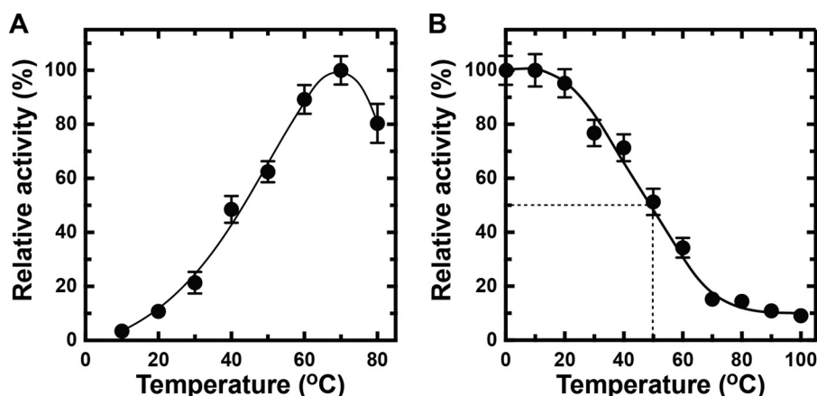
FIGURE 7. Effects of DTT on the temperature dependence and heat stability of NitAly. A, temperature dependence of alginate lyase activity of rNitAly in the presence of DTT. Assays were performed as described for Fig. 5A, except that DTT was added to the reaction mixture at a final concentration of 5 mM. Relative activity at 100% was equivalent to 1,590 units/mg. B, heat stability of rNitAly in the presence of DTT. Samples were preincubated as described for Fig. 6A, except that DTT was added at a final concentration of 5 mM. Assays were performed as described in A at 50 °C. Relative activity at 100% was equivalent to 1,080 units/mg. All assays were repeated three times, and the data are shown as mean \pm S.D.
