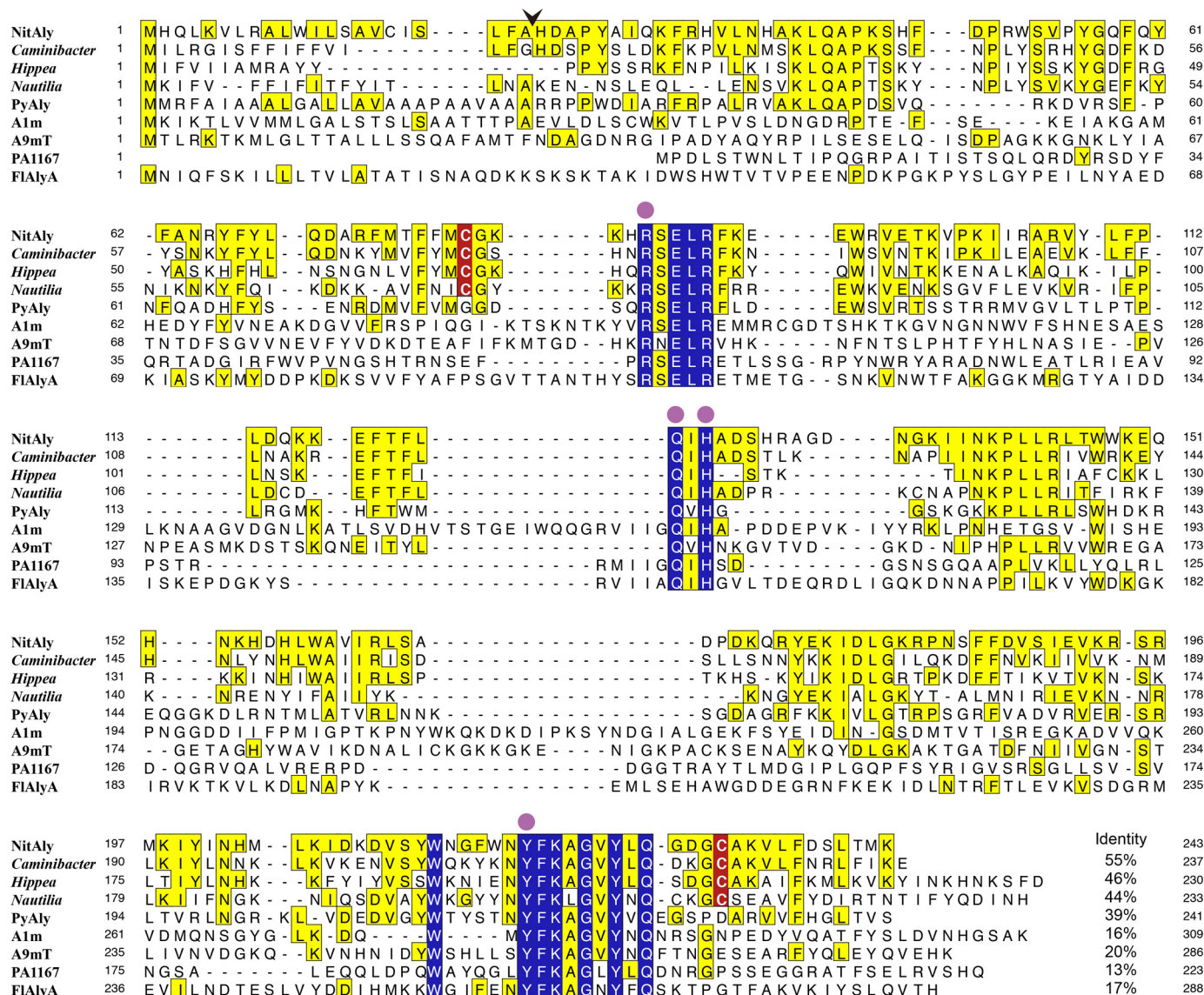
FIGURE 1. Comparison among the amino acid sequences of NitAly, its homologous proteins, and several characterized family PL-7 alginate lyases. NitAly, Nitratiruptor sp. SB155-2 hypothetical protein NIS_0185 (GenBank TM accession no. WP_012081562); Caminibacter, C. mediatlanticus hypothetical protein (GenBank TM accession no. WP_007473671); Hippea, H. jasoniae hypothetical protein (GenBank TM accession no. WP_051904545); Nautilia, N. profundicola predicted alginate lyase (GenBank TM accession no. WP_015901805); PyAly, P. yezoensis alginate lyase PyAly (GenBank TM accession no. BA166416) (39); PA1167, P. aeruginosa PAO1 alginate lyase PA1167 (GenBank TM accession no. AAG04556) (15); A1m, Agarivorans sp. JAM-A1m alginate lyase A1m (GenBank TM accession no. AB426616) (31); A9mT, Vibrio sp. alginate lyase A9mT (GenBank TM accession no. AB473598) (25); FlAlyA, Flavobacterium sp. UMI-01 alginate lyase FlAlyA (18). Residues invariant among all listed proteins are indicated with blue boxes. Residues identical with those of NitAly are indicated with yellow boxes. Cys-80 and Cys-232 in NitAly and their corresponding conserved Cys residues in other proteins are highlighted with red. An arrowhead shows the cleavage site of the signal peptide in NitAly predicted by the SignalP 3.0 software program. Catalytic residues proposed in PL-7 alginate lyases (15, 21, 65) are shown by solid circles. The level of identity of each other protein with NitAly is shown at the end of each sequence, respectively.
