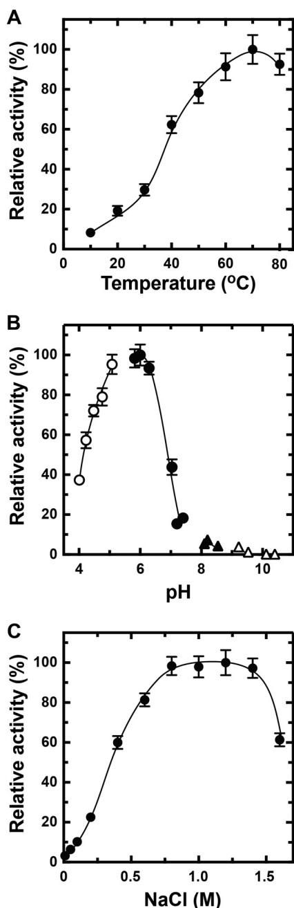
FIGURE 5. Effects of temperature, pH, NaCl, and divalent metals on rNitAly activity. A, temperature dependence of alginate lyase activity of rNitAly. Enzyme reactions were conducted in a solution containing 10 mM sodium phosphate (pH 6.0), 1 mM NaCl, 0.1 mg/ml BSA, 0.005 mg/ml rNitAly, and 0.5% (w/v) polyM for 15 min at the indicated temperatures. Relative activity of 100% was equivalent to 1,620 units/mg. B, pH dependence of the alginate lyase activity of rNitAly. Assays were performed as described for A, except that reaction mixtures were incubated at 50 °C for 15 min in 10 mM sodium acetate for pH 4.0–5.1 (open circles), 10 mM sodium phosphate for pH 5.7–7.4 (closed circles), 10 mM Tris-HCl for pH 8.1–8.5 (closed triangles), and 10 mM glycine-NaOH for pH 9.2–10.4 (open triangles). Relative activity at 100% was equivalent to 1,230 units/mg. C, NaCl dependence of the alginate lyase activity of rNitAly. Assays were performed as described for A at 50 °C, except that different concentrations of NaCl were used as indicated. Relative activity at 100% was equivalent to 1,430 units/mg.
