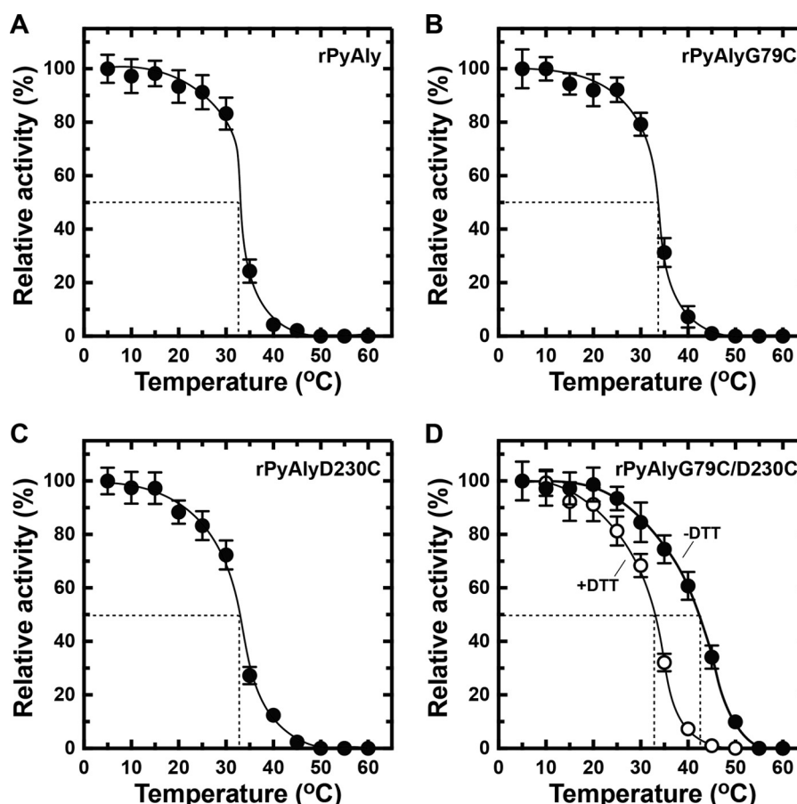
FIGURE 11. Effects of replacing residue(s) of rPyAly with cysteine on its heat stability. Enzyme solution containing 10 mM sodium phosphate (pH 8.0), 0.1 M NaCl, and 0.15 mg/ml rPyAly (A), rPyAlyG79C (B), rPyAlyD230C (C), or rPyAlyG79C/D230C (D, -DTT) was incubated for 30 min at the indicated temperatures and placed on ice. For rPyAlyG79C/D230C, 5 mM DTT was also added during incubation (D, +DTT). Enzyme activity was then assayed as described for Fig. 10 at 30 °C. Relative activity at 100% was equivalent to 1,730 units/mg (A), 1,620 units/mg (B), 1,540 units/mg (C), 1,600 units/mg (D, -DTT), and 1,420 units/mg (D, +DTT). All assays were repeated three times, and the data are shown as mean \pm S.D.
