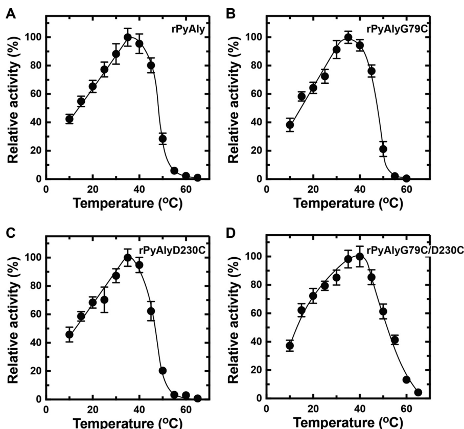
FIGURE 10. Effects of replacing the residues of rPyAly with cysteine on its temperature dependence. Enzyme reactions were conducted in a solution containing 10 mM sodium phosphate (pH 8.0), 0.1 M NaCl, 0.1 mg/ml BSA, 0.25% (w/v) polyM, and 0.005 mg/ml rPyAly (A), rPyAlyG79C (B), rPyAlyD230C (C), or rPyAlyG79C/D230C (D) for 15 min at the indicated temperatures. Relative activity at 100% was equivalent to 1,820 units/mg (A), 1,740 units/mg (B), 1,710 units/mg (C), and 1,780 units/mg (D). All assays were repeated three times, and the data are shown as mean \pm S.D.
