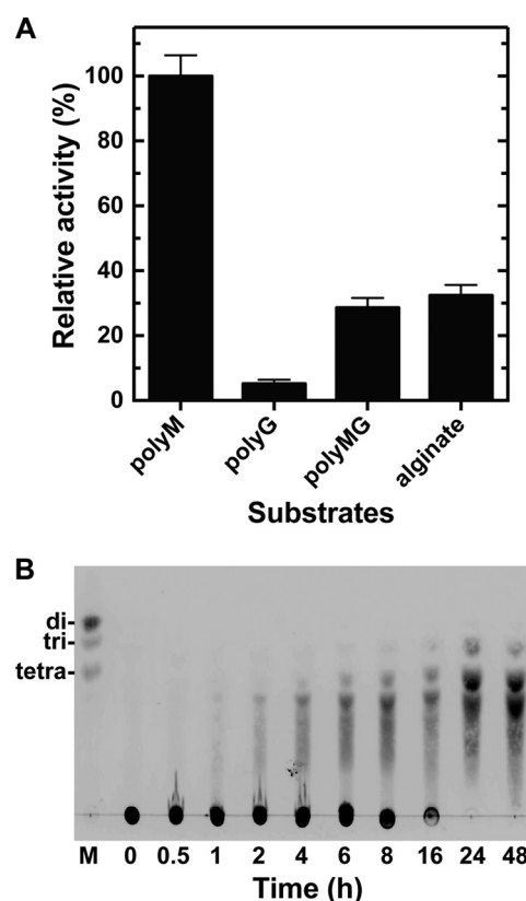
FIGURE 4. Substrate preferences of rNitAly and degradation products. A, substrate preferences of rNitAly. Enzyme reactions were conducted in a solution containing 10 mM sodium phosphate buffer (pH 6.0), 1 M NaCl, 0.1 mg/ml BSA, 0.005 mg/ml rNitAly, and 0.5% (w/v) substrate (polyM, polyG, polyMG, or sodium alginate) at 50 °C for 15 min. A relative activity of 100% was equivalent to 1,290 units/mg. Assays were done three times, and the data were shown as mean \pm S.D. B, thin layer chromatography analysis of the degradation products of polyM following incubation with rNitAly. The enzyme reaction was conducted using polyM as the substrate under the same conditions described for A, and was stopped by the addition of 4 volumes of ice-cold ethanol at the indicated time point.
