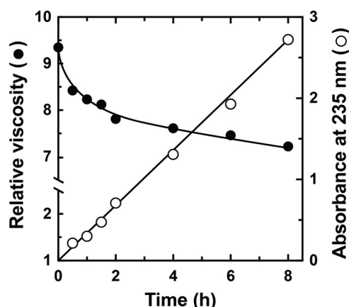
FIGURE 3. Evaluation of an alginate lyase activity of rNitAly. Relative viscosity (closed circles) and absorbance at 235 nm (open circles) were measured in a mixture of 10 mM sodium phosphate (pH 6.0), 1 M NaCl, 0.1 mg/ml BSA, 1% (w/v) sodium alginate, and 0.005 mg/ml rNitAly at 30 °C at the indicated time points.
