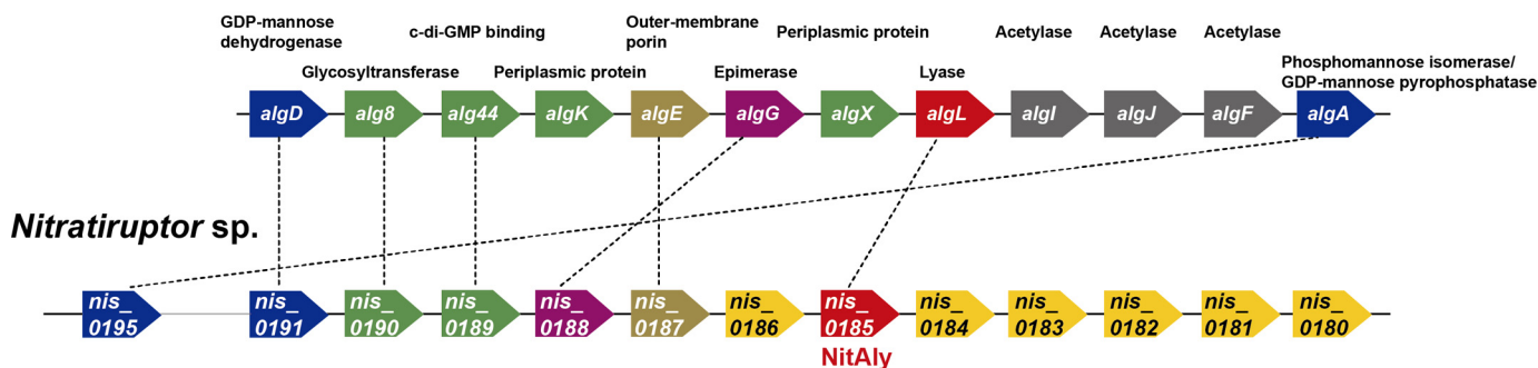
FIGURE 12. Assignment of genes in the alginate biosynthesis operon of P. aeruginosa and their homologs in Nitratiruptor sp. SB155-2. Genes encoding proteins with homology between P. aeruginosa and Nitratiruptor sp. SB155-2 are connected by dotted lines. Each pentagon is classified by a different color based on known function in P. aeruginosa as follows: blue, precursor biosynthesis; green, alginate polymerization; brown, alginate export; violet, epimerization of mannuronic acid to guluronic acid; red, alginate degradation; gray, O-acetylation. Yellow pentagons show genes with unidentified functions in Nitratiruptor sp. SB155-2.
