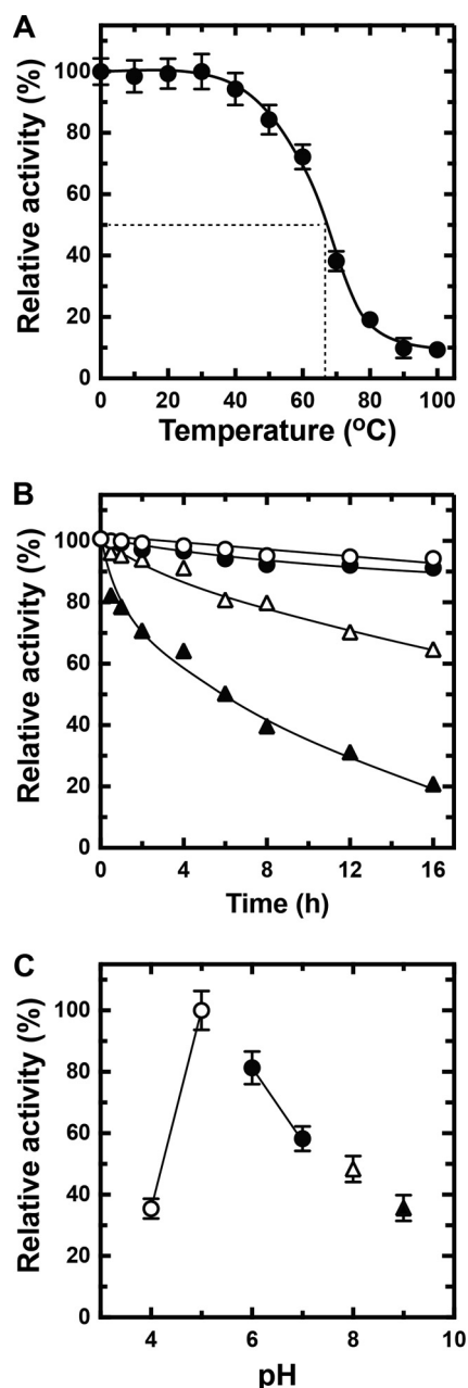
FIGURE 6. Effects of temperature and pH on rNitAly stability. A, heat stability of rNitAly. For this assay, 0.2 mg/ml rNitAly in 10 mM sodium phosphate (pH 6.0) and 1 M NaCl were incubated for 30 min at the indicated temperatures and placed on ice. Enzyme activity was then assayed as described in Fig. 5A at 50 °C. Relative activity at 100% was equivalent to 1,230 units/mg. B, effects of time extension of heat treatment on the heat stability of rNitAly. For this assay, 0.2 mg/ml rNitAly in 10 mM sodium phosphate (pH 6.0) and 1 M NaCl were incubated for the indicated time at 20 °C (open circles), 30 °C (closed circles), 40 °C (open triangles), and 50 °C (closed triangles) and placed on ice. Assays were performed as described for A. Relative activity at 100% was equivalent to 1,210 units/mg. C, pH stability of rNitAly. For this assay, 0.2 mg/ml rNitAly in 10 mM sodium phosphate (pH 6.0) and 1 M NaCl was dialyzed against 1,000 volumes of 1 M NaCl and 10 mM sodium acetate (pH 4.0 or 5.0) (open circles), 10 mM sodium phosphate (pH 6.0 or 7.0) (closed circles), 10 mM Tris-HCl (pH 8.0) (open triangle), and 10 mM glycine-KOH (pH 9.0) (closed triangle) at 4 °C for 8 h. Assays were performed as described for A. Relative activity at 100% was equivalent to 1,410 units/mg. All assays were repeated three times, and the data are shown as mean \pm S.D.
