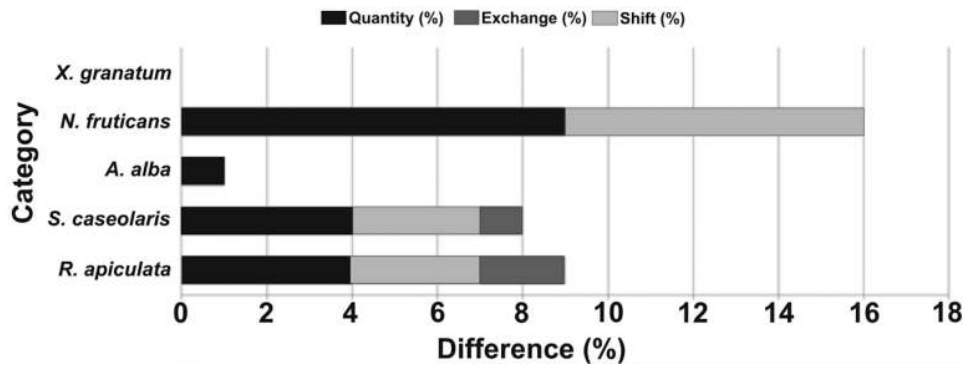
Figure 3 Pontius matrix. Quantity, Exchange and Shift differences in species-level mangrove supervised classification at Brunei Bay (Genus names: R, Rhizophora ; S, Sonneratia ; N, Nypa and X, Xylocarpus ). The X-axis refers to the difference (%) in each mangrove category of the study area.
