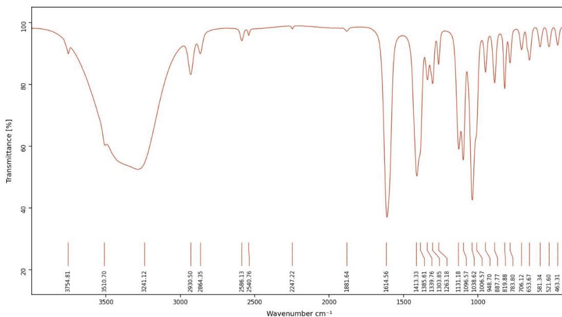
Figure 3.7: FTIR Spectra of Sodium Alginate
