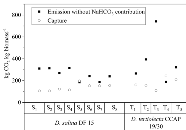
Fig. 9 \text{CO}_2 -eq emission from the LCIA and the hypothetical \text{CO}_2 captured by D. salina and D. tertiolecta for the proposed scenarios
