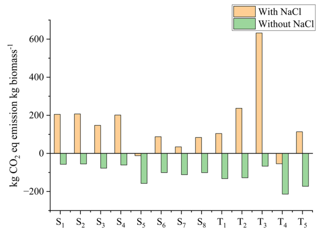
Fig. 10 \text{CO}_2 -eq emissions by D. salina and D. tertiolecta for the proposed scenarios with and without NaCl contribution (assuming the use of brine from desalination plants). \text{NaHCO}_3 contribution was neglected in both conditions (with and without NaCl contribution) as carbon would be supplied by \text{CO}_2
