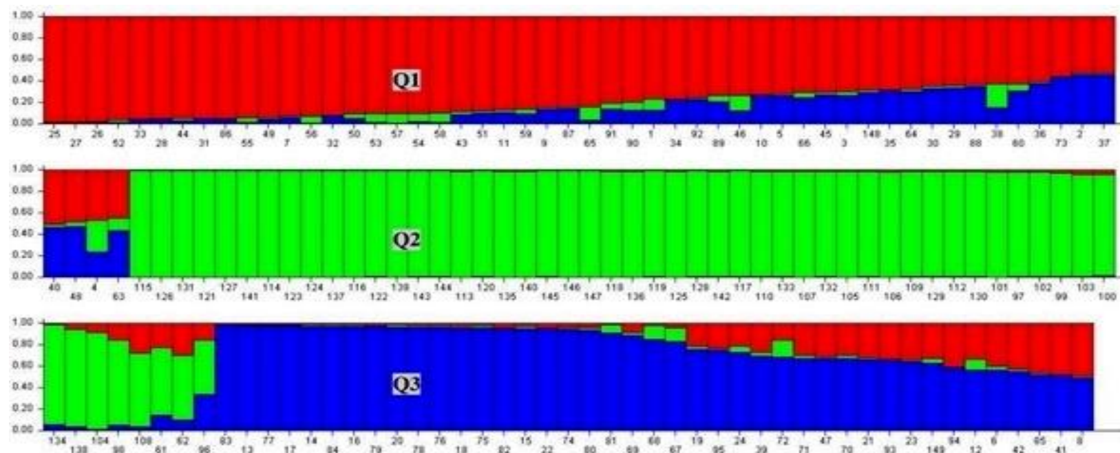
Figure 6. Alfalfa population structure among 147 progeny of BC 3 and their two parents analyzed with 15 SSR markers assuming Three clusters, K = 3: Population Q1 (Red bars, n=51), Population Q2 (Green bars, n=53) and Population Q3 (Blue bars, n=40). X-axis indicates the name of the genotypes and the numbers on the y-axis denote genetic proportion in different groups.
