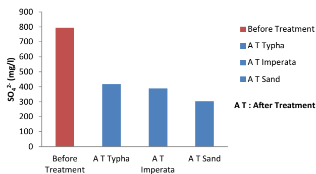
Fig. 13 Results of sulfate before and after treatment
