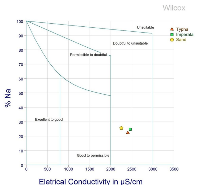
Fig. 27 Wilcox diagram for treated waters
