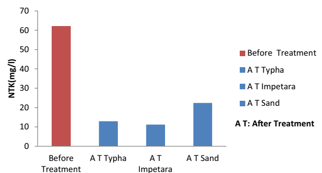
Fig. 10 Results of Kjeldahl nitrogen before and after treatment
