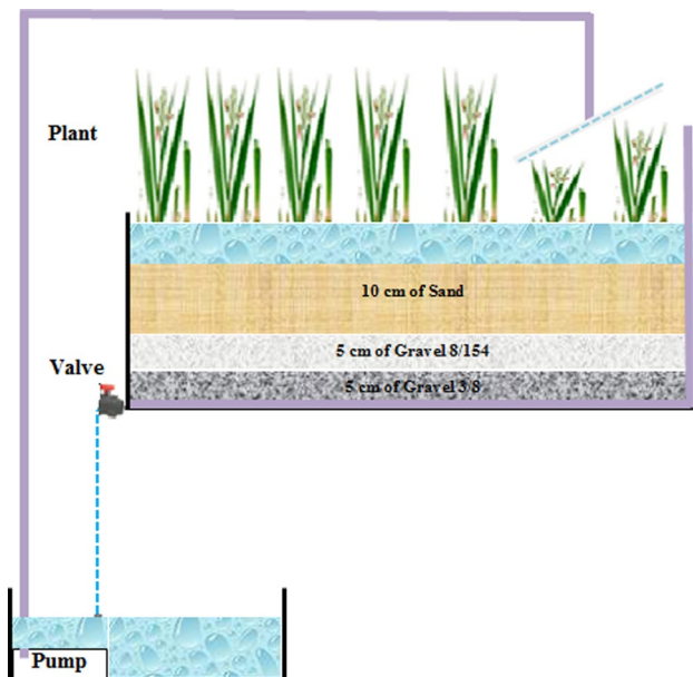
Fig. 1 Schema of the experimental pilot (Bendida 2012)
