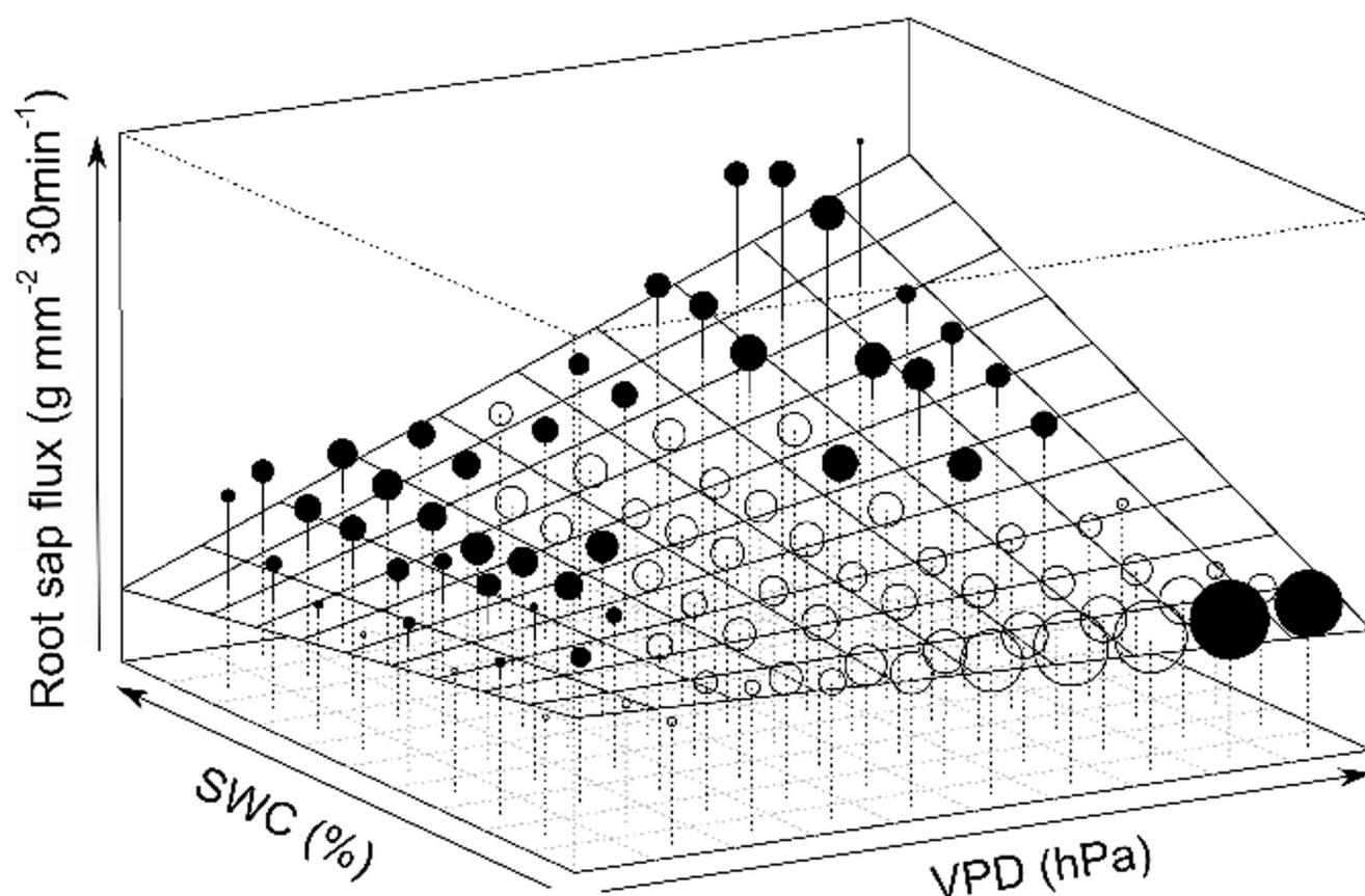
Fig. 5 Effects of SWC and VPD on root sap flux density (surface area) in Eriotheca ruizii , for daytime and radiation intensity being at their average (crown status dummy-coded and then centered, R^2=0.19 , P<0.001 ). Dot volume depicts the number of samples per cell. Values below the fitted model surface are depicted as open, values above the
