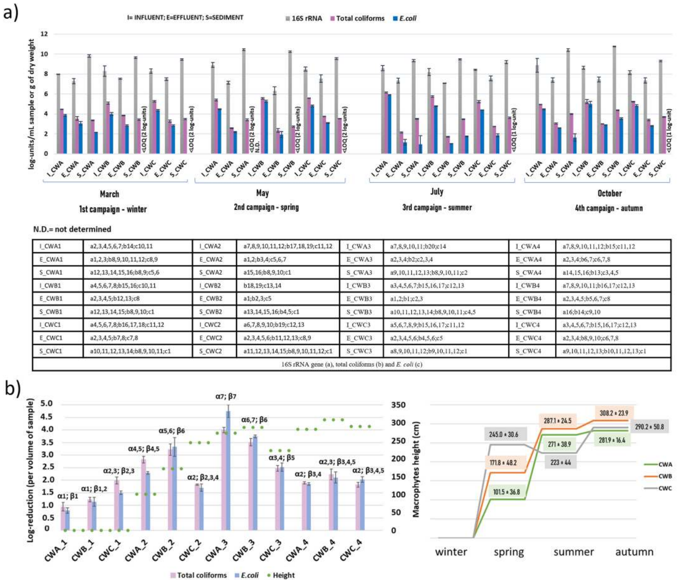
Fig. 2. a) Total coliforms and E. coli colony forming units per volume of sample (log CFU/mL or g of dry weight) and bacterial load based on 16S rRNA gene quantification by qPCR (log gene copy/mL or g of dry weight), in influent (I), effluent (E) and sediment (S) samples of the three CWs (A, B and C). b) Enterobacterial reduction values (log CFU/volume) for the three different CWs (A, B and C) [influent (I) - effluent (E) counts] and macrophytes height (cm) across the four sampling dates (1-winter, 2-spring, 3-summer, and 4-autumn). The different Tukey's groups for 16S rRNA gene, total coliforms and E. coli by CW are displayed in the table.
