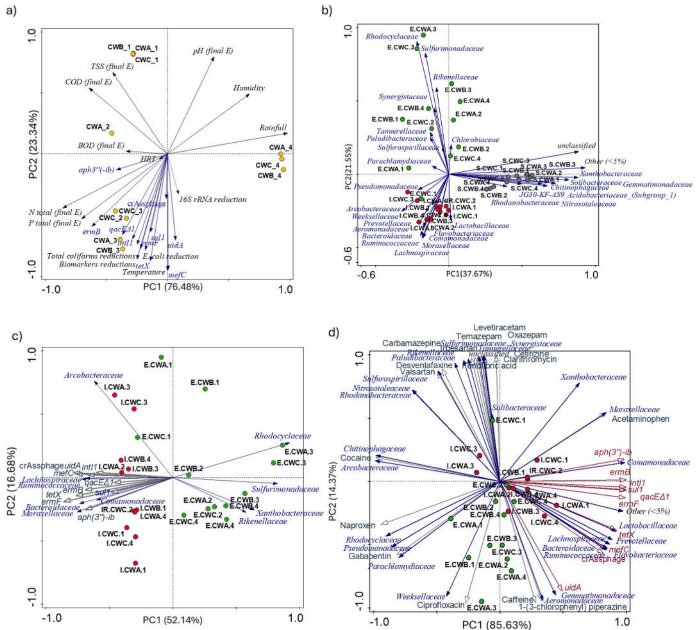
Fig. 6. Unconstrained principal component analysis (PCA) of a ) biomarkers ( int1 , uidA , crAssphage , sul1 , ermB , ermF , mefC , qacEΔ1 , tetX and aph(3'')-Ib ), 16S rRNA gene (log-units gene copy/mL), total coliforms and E. coli reductions (log-units CFU/mL), N and P total (final effluent) (mg/L), rainfall (mm), humidity (%), and temperature (°C); b ) bacterial community composition, expressed as family relative abundance (> 5%) between the influent (I), effluent (E), and sediments (S) samples; c ) qPCR biomarker quantification (gene copy/mL of sample) and the most 10 most representative bacterial families; and d ) qPCR biomarkers quantification (gene copy/mL of sample), the most abundant bacterial families and OMPs for the three CWs (A, B, and C) in the different seasons (1-winter, 2-spring, 3-summer, and 4-autumn).
