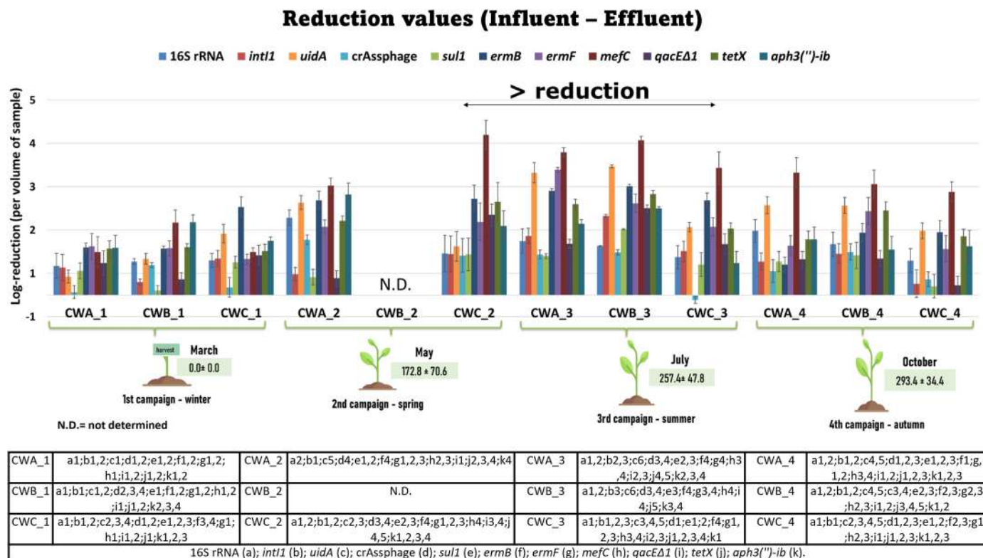
Fig. 3. Reduction values (log-units/mL) of 16S rRNA gene and biomarkers for genetic recombination ( int1 ), fecal contamination ( uidA and crAssphage ) and antibiotic resistance ( sul1 , ermB , ermF , mefC , qacED1 , tetX , aph3(III)-ib ) [influent (I) - effluent (E)] and macrophyte height (cm) in the four sampling dates. The different Tukey's groups for the different genes are displayed in the table.
