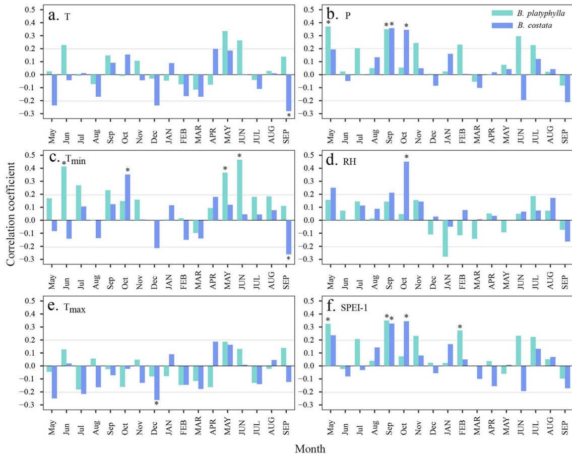
Fig. 3 Correlation coefficients between the tree-ring indices of B. platyphylla (1963–2017) and B. costata (1964–2016) and major monthly climate factors; T: monthly mean temperature; T_{\min} : monthly minimum temperature; T_{\max} : monthly maximum temperature; P:
