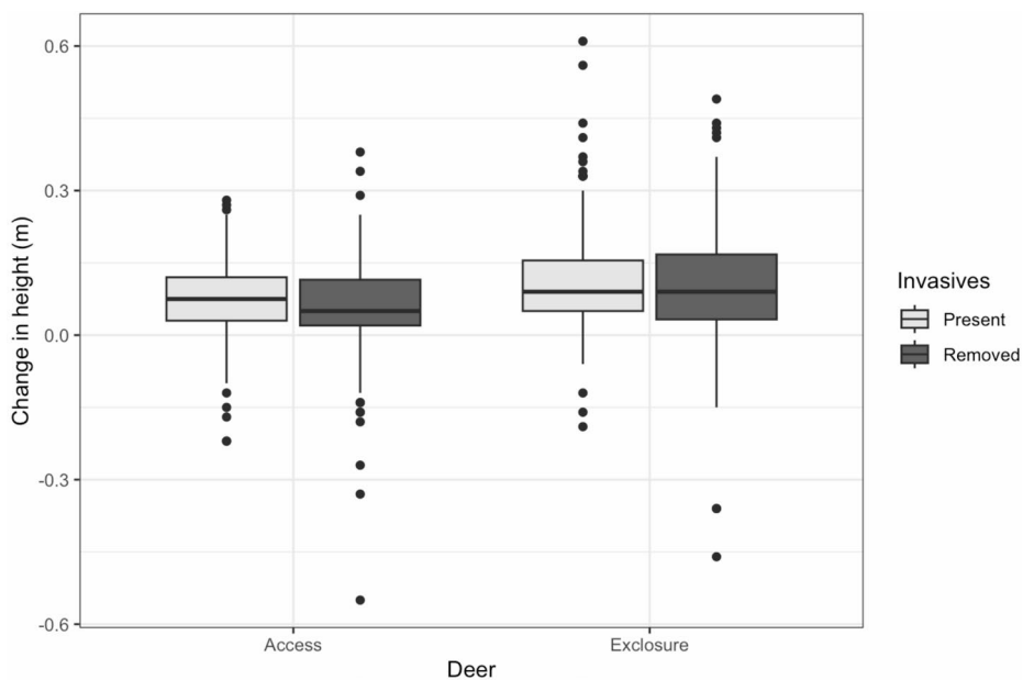
Fig. 5 Boxplot of change in height of natural regeneration by deer and invasive treatment between June 2022 and June 2025. Heights analyzed for each native tree seedling 30\text{ cm} < \text{ht} < 2.5\text{ m} still alive in 2025
