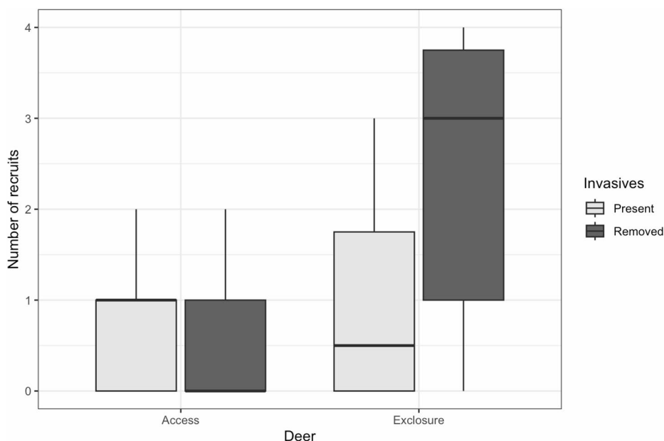
Fig. 7 Boxplot of recruitment of native seedlings per plot by 2025, excluding F. americana , by deer and invasive treatments. New recruits were native seedlings that passed the 0.3 m height threshold in each plot after June 2022
