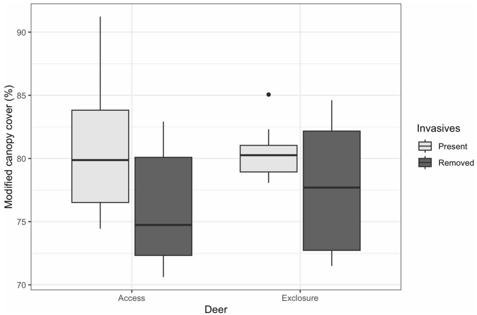
Fig. 3 Boxplot of Modified Canopy Cover index values at 0.3 m by deer and invasive treatment. Canopy photographs were taken in the center of each plot at 0.3 m above ground and analyzed in the GLAMA app
