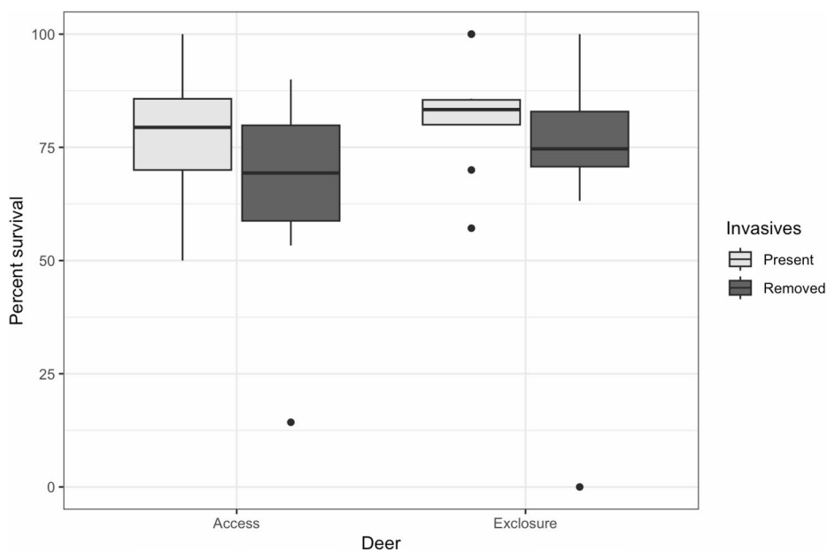
Fig. 4 Boxplot of percent survival of all natural regeneration. Percent survival is the percent of naturally occurring seedlings tagged in June 2022 in a plot that were still living by June 2025
