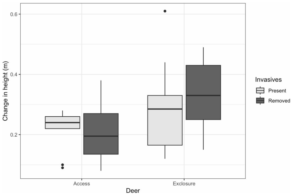
Fig. 6 Boxplot of change in height (2022–2025) for the natural regeneration seedling in each plot with the greatest height growth
