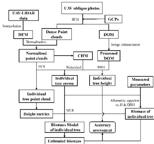
FIGURE 1. Flowchart of individual tree parameters estimation. SfM: structure from motion; GCPs: ground control points; DEM: digital elevation model; DOM: digital orthophoto map; PCS: point cloud segmentation; MRS: multi-resolution segmentation; MLR: multiple linear regression; H: tree height; DBH: diameter at breast height.
