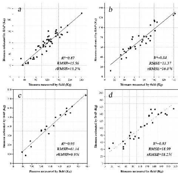
FIGURE 11. Accuracy verification results of the optimal models. (a), (b), (c) and (d) are the verification results of the biomass of mature larch, young larch, mature Chinese pine and young Chinese pine, respectively.
