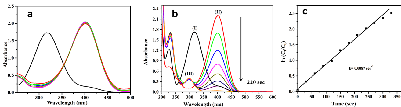
Fig. 8 (a) UV-Vis spectrum of 4-NP with NaBH 4 as the sole catalyst. (b) UV-Vis spectrum of 4-NP with a PdNPs catalyst in the presence of NaBH 4 , showing the absorption maximum corresponding to (I) 4-NP,
