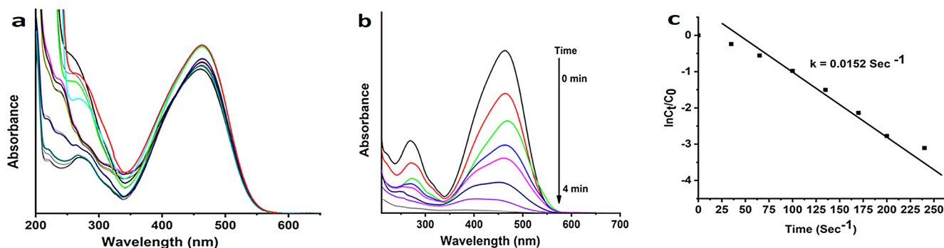
Fig. 9 UV -Visible Absorption spectra of (a) MO in the presence of NaBH 4 and in the absence of PdNPs, (b) Time-dependent MO reduction with NaBH 4 and PdNPs catalysts, and (c) Linear plot of (C_t/C_0) vs. time
