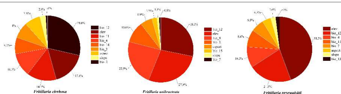
FIGURE 3 | The contribution rate of each environment variable to the modeling of MaxEnt.
