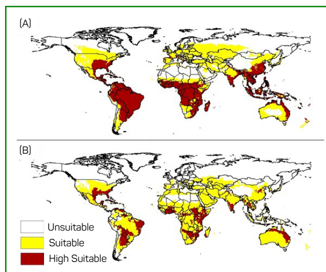
Figure 2 - (A) New model for Amaranthus palmeri and (B) Model proposed by Kistner and Hatfield (2018) for the current climate
