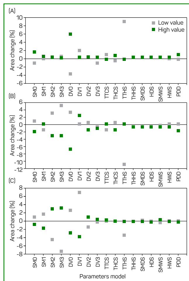
Figure 6 - Changes in (A) unsuitable, (B) suitable, and (C) highly suitable areas for the potential distribution of Amaranthus palmeri when the sensitivity analysis was performed based on 17 CLIMEX parameters, with greater sensitivity in EI. The values for the various parameters used are those given in Table 1
