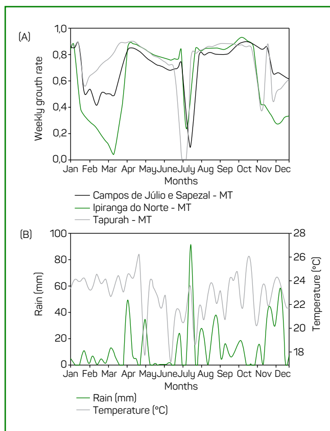
Figure 5 - (A) Weekly growth index (GIW) of Amaranthus palmeri in the municipalities of Campos de Júlio, Sapezal, Ipiranga do Norte, and Tapurah, state of Mato Grosso. (B) Precipitation and temperature index for these locations
