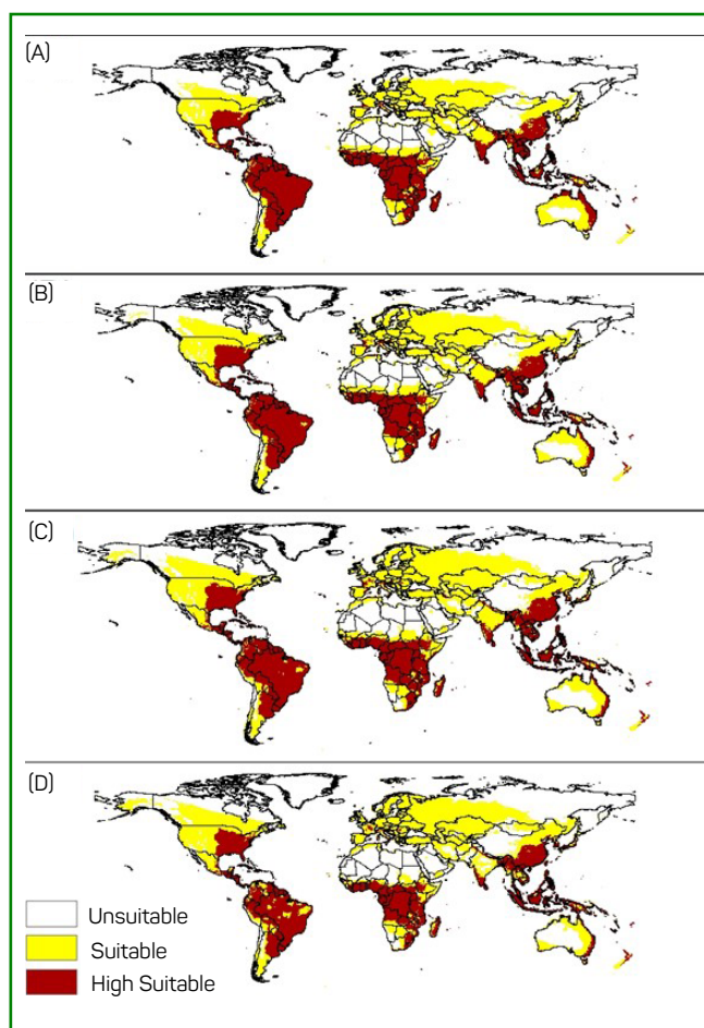
Figure 3 - Potential distribution of Amaranthus palmeri for current climate (A) and 2050 (B), 2070 (C), and 2100 (D) climate change in the world
