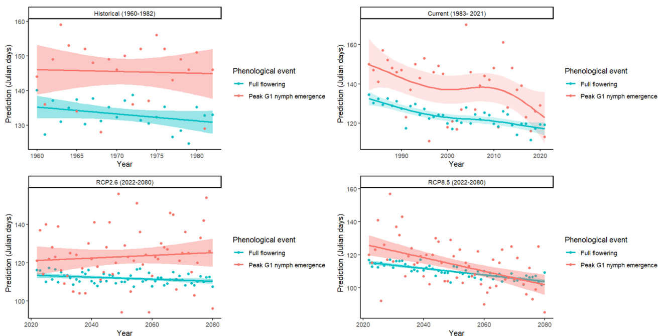
Fig. 4 Phenological shift in full flowering time (Julian days) for cv. Conference pear trees ( Pyrus communis ) and Cacopsylla pyri G1 peak nymph abundance date, depending on year (1960–2080) and RCP scenario (RCP2.6 and RCP8.5)
