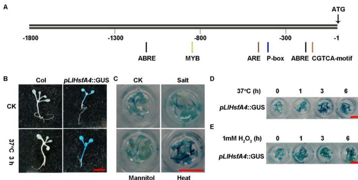
Figure 3. Expression analysis of HsfA4 using pLIHsfA4::GUS transgenic Arabidopsis . (A) Cis-element analysis of LIHsfA4 promoter using PLACE data. GUS staining of pLIHsfA4::GUS transgenic Arabidopsis seedlings were treated with different abiotic stresses: heat stress in (B–D), salt (150 mM NaCl) and osmosis (300 mM Mannitol) in (C) and ROS (1 mM H_2O_2 ) in (E). Bar: 50 mm.
