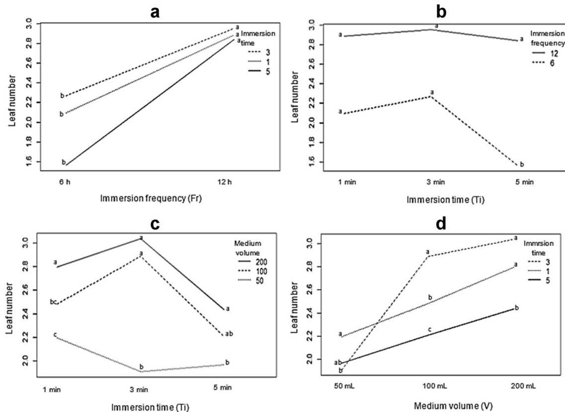
Figure 2. First-order interactions, between a, b immersion frequency with immersion time (Fr:Ti) and c, d immersion time with culture medium volume (Ti:V) for the variable leaf number in C. palmata micropropagation using temporary immersion system. Means
