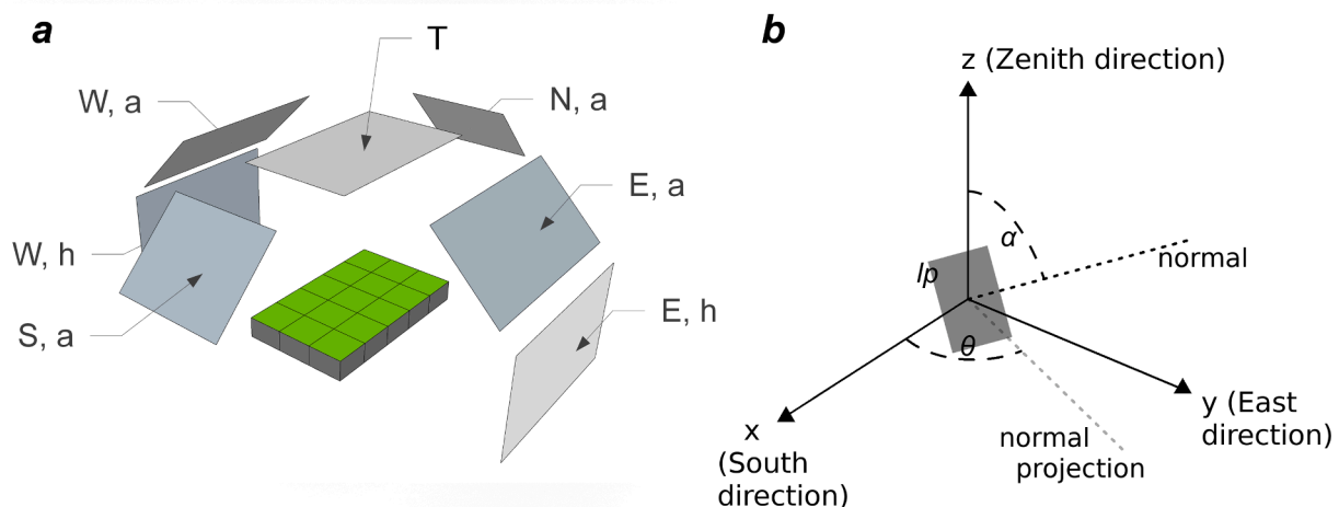
Fig. 3. A. perspective planes used for photographing the studied plants which grew in multipot trays; capital letters denote different sides from which the photos were taken: N – north, S – south, W – west, E – east, T – top; small letters designate horizontal (h) or angled (a) perspective; b. Definition of leaf orientation: lp – leaf plate, \Theta – leaf azimuth and \alpha – leaf inclination.
