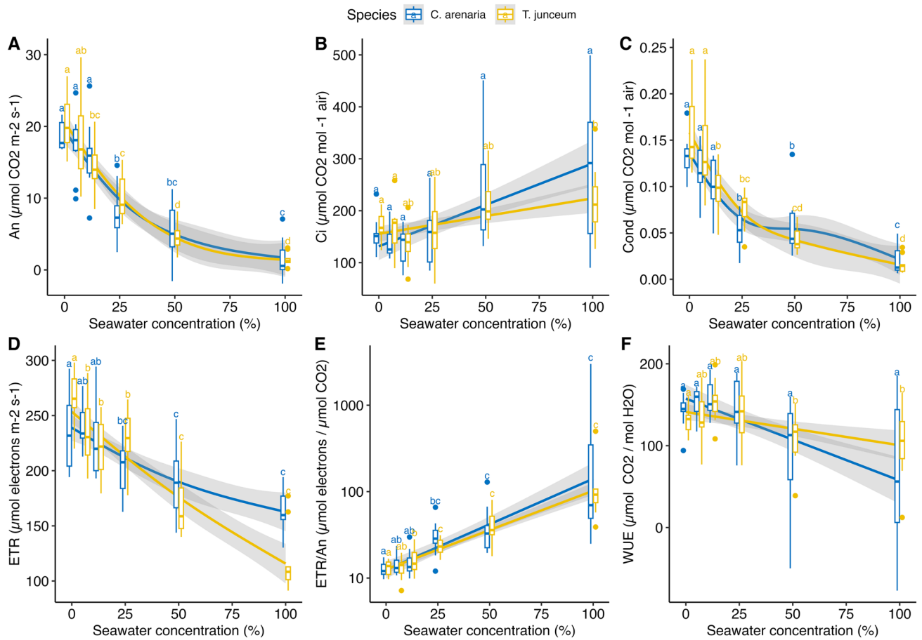
Fig. 3 Seawater effect on gas exchange measurements for Calamagrostis arenaria (3l) and Thinopyrum junceum . Assimilation rate (An), Inter-cellular \text{CO}_2 (Ci), Stomatal conductance (gs), electron
