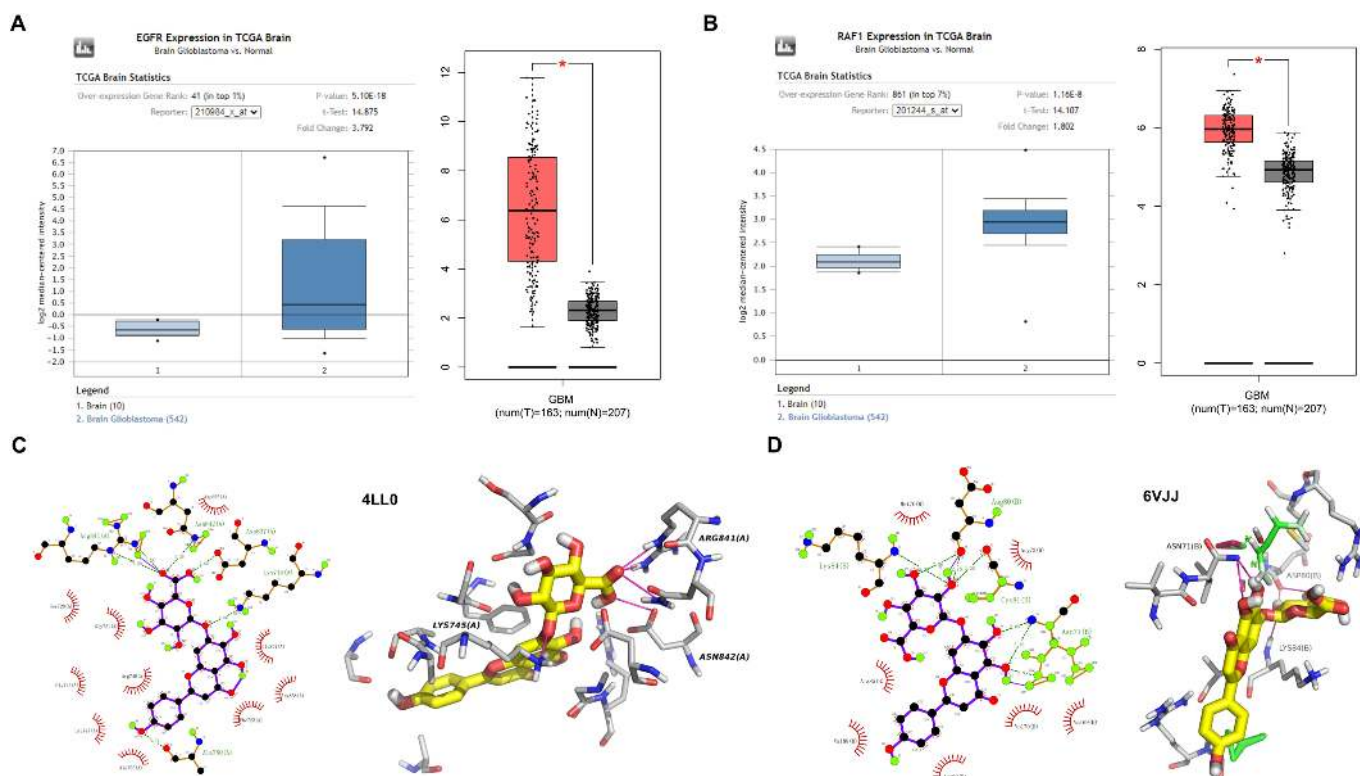
Figure 6. Molecular docking of scutellarin and its potential targets. (A and B) Expression of EGFR and RAF1 in Oncomine and GEPIA databases. (C) The 2D and 3D representation of the binding of scutellarin with EGFR (4LL0). (D) The 2D and 3D representation of the binding of scutellarin with RAF1 (6VJJ).
