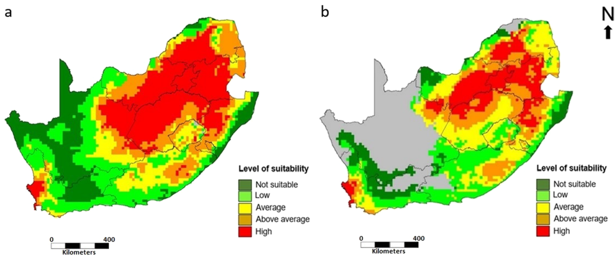
Fig. 5 Potential distribution of Zygodontia piceicollis (a) and Zygodontia signatipennis (b) in South Africa, using MaxEnt modelling
