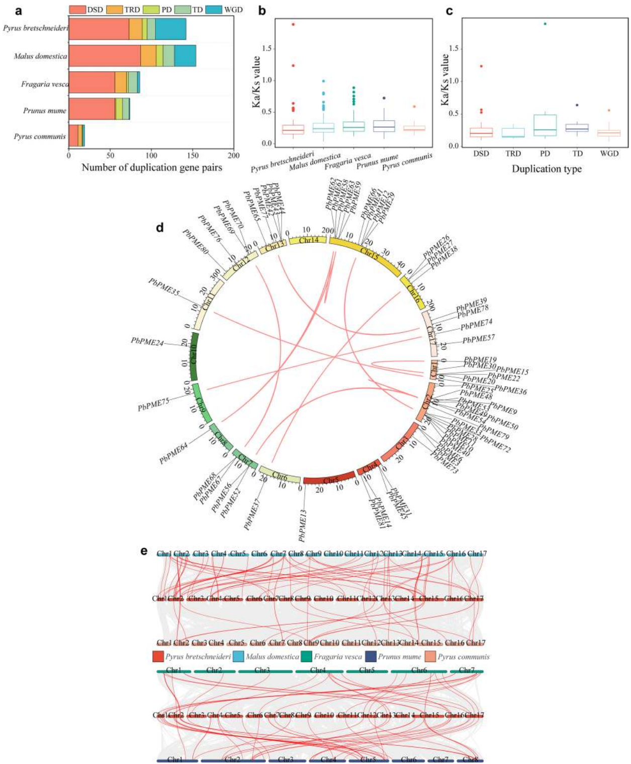
Fig. 2 Gene-duplication modes, Ka/Ks values, gene locations, and collinearity analysis of the Pectin methylesterase (PME) gene family. (a) Various modes of gene duplication, with the x-axis representing the number of duplicated gene pairs and the y-axis denoting the species. (b) Ka/Ks values across five Rosaceae species. (c) Ka/Ks values corresponding to different duplication modes in Pyrus bretschneideri . (d) Gene locations in P. bretschneideri and collinearity analysis, displaying genes distributed across different chromosomes. Red lines represent syntenic gene pairs. (e) Collinearity analysis comparing P. bretschneideri with four Rosaceae species. DSD, dispersed duplication; TRD, transposon duplication; PD, proximal duplication; TD, tandem duplication; WGD, whole genome duplication; Ka, nonsynonymous substitutions per nonsynonymous site; Ks, synonymous substitutions per synonymous site
