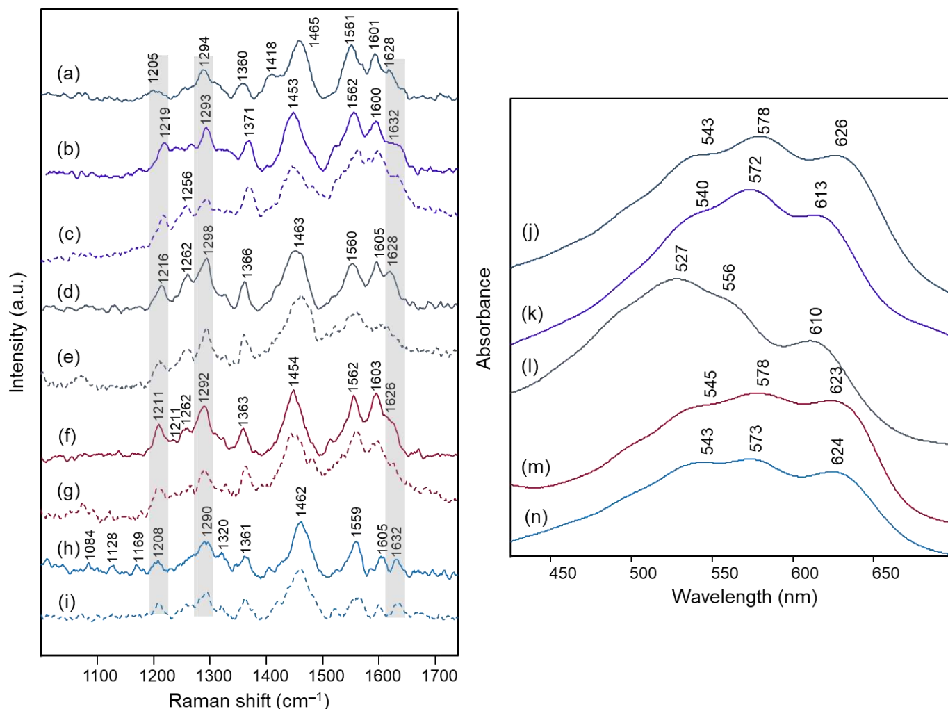
Figure 3. Micro-Raman spectra ( \lambda_{\text{exc}} 457 nm) of: (a) Agapanthus intact petals; (b) Anemone coronaria intact petals and (c) anthocyanin extract; (d) Campanula portenschlagiana intact petals and (e) anthocyanin extract; (f) Cineraria intact petals and (g) anthocyanin extract; (h) Platycodon intact petals and (i) anthocyanin extract. Visible spectra acquired in microscopic reflection mode on intact petals of: (j) Agapanthus ; (k) Anemone coronaria ; (l) Campanula portenschlagiana ; (m) Cineraria ; (n) Platycodon . For easier interpretation, the same line color was used for all spectra corresponding to the same flower. Anthocyanin extracts were examined in aqueous solution at a pH value ranging from 4.5 to 6. The grey bars highlight the bands that were found to be characteristic of the 3,7-di-O substitution pattern in the benzopyrylium moiety. Legend: (solid lines) petals; (dashed lined) anthocyanin extract.
