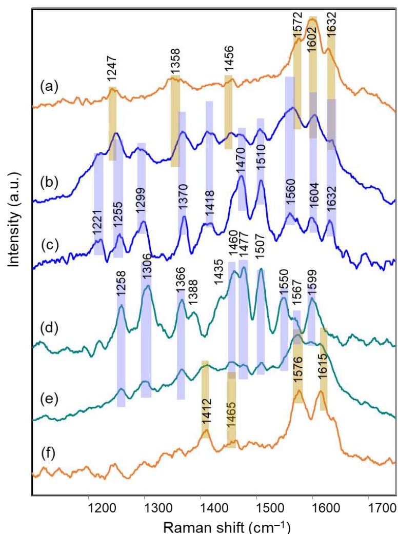
Figure 8. Micro-Raman spectra ( \lambda_{\text{exc}} 457 nm) of: (a) flavonol fraction isolated from the petals of Cerastostigma plumbaginoides ; (b) intact petal of Cerastostigma plumbaginoides ; (c) anthocyanin fraction isolated from the petals of Cerastostigma plumbaginoides in aqueous solution at pH 6; (d) anthocyanin fraction isolated from the petals of Plumbago capensis in aqueous solution at pH 5.5; (e) intact petal of Plumbago capensis ; (f) flavonol fraction isolated from the petals of Plumbago capensis . Legend: (orange lines) flavonols; (light blue lines) anthocyanins and intact petals. The vertical bars allow to recognize in the spectra of the petals the bands due respectively to flavonols and anthocyanins.
