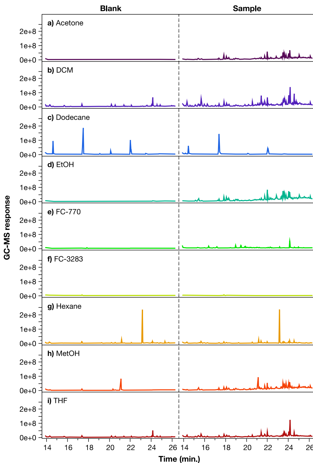
Fig. 2 GC chromatograms of pure solvents (left panels) and of agarwood extracts (right panels) from the preliminary extraction-solvent experiment with acetone, dichloromethane (DCM), dodecane, ethanol (EtOH), FC-770, FC-3283, hexane, methanol (MetOH), and tetrahydrofuran (THF)
