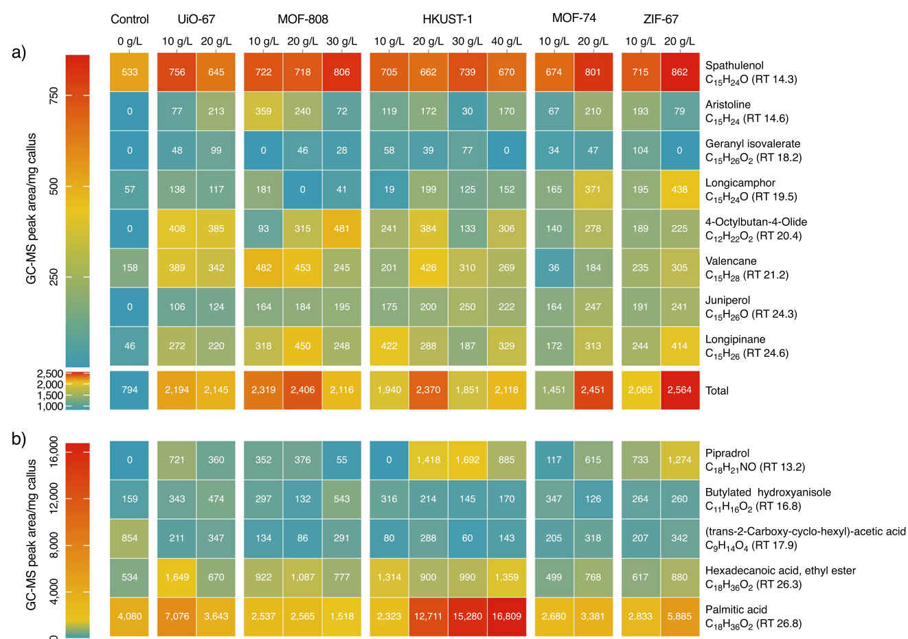
Fig. 3 Relative quantification (as GC–MS peak area/mg callus) of various (a) fragrant metabolites and (b) other prominent compounds produced by A. crassna callus cultures following different MOF treatments. RT refers to the GC retention time in minutes. Numbers inside boxes represent mean values of four replicates (n = 4). The highest value in each row is underlined
