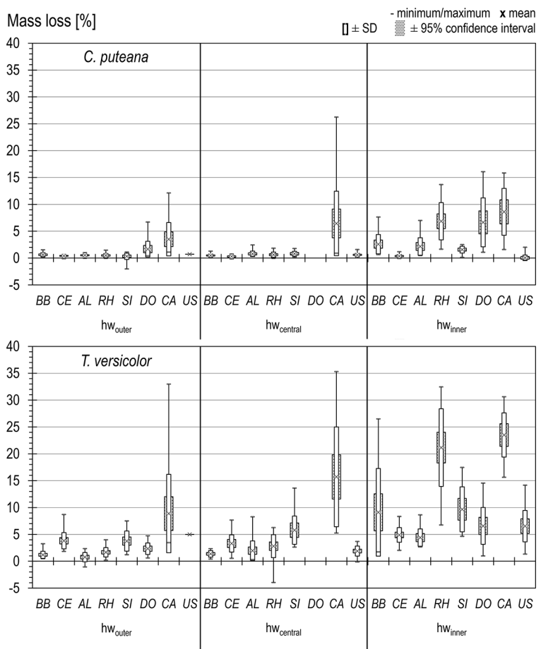
Fig. 3 Mass loss of different black locust origins and stem sections due to fungal decay after 16 weeks of incubation with Coniophora puteana and Trametes versicolor : No specimens of hw central from DO were available
