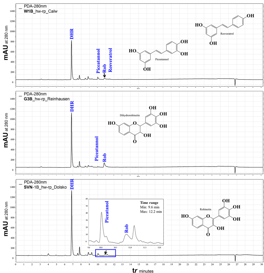
Fig. 4 HPLC-PDA chromatograms of acetone extracts of black locust monitored at 280 nm. The phenolic compounds targeted were dihydroresveratrol (DHR) and robinetin (Rob), as the high natural durability of the heartwood of black locust is associated with the presence of resveratrols. Calw (W1B), Reinhausen (G3B), and Dolsko (SVN). HPLC of the heartwood extracts gave the following elution order: Dihydroresveratrol (DHR), t_r = 6.9 min; Picetannol, t_r = 10.0 min; Robinetin (Rob), t_r = 10.9 min, and Resveratrol, t_r = 11.5 min. HPLC run time was 30.2 min
