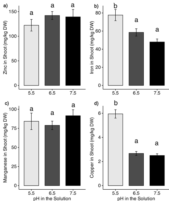
Fig. 7 Iron, zinc, manganese, and copper concentrations in plant shoots of Bornmuellera in Experiment 2 are shown in panels (a) Zn, (b) Fe, (c) Mn, and (d) Cu. Bars represent the standard error of the mean n=6 . Means labelled with different letters indicate significant differences at p<0.05 using Fisher's exact test
