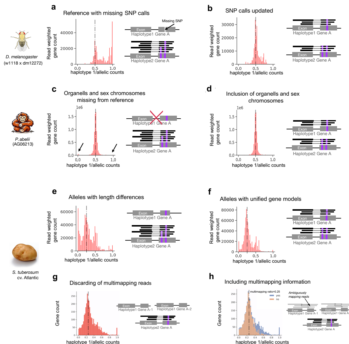
Figure 2: Examples of annotation and assembly errors causing bias that can be identified and corrected with long-read RNA-seq
