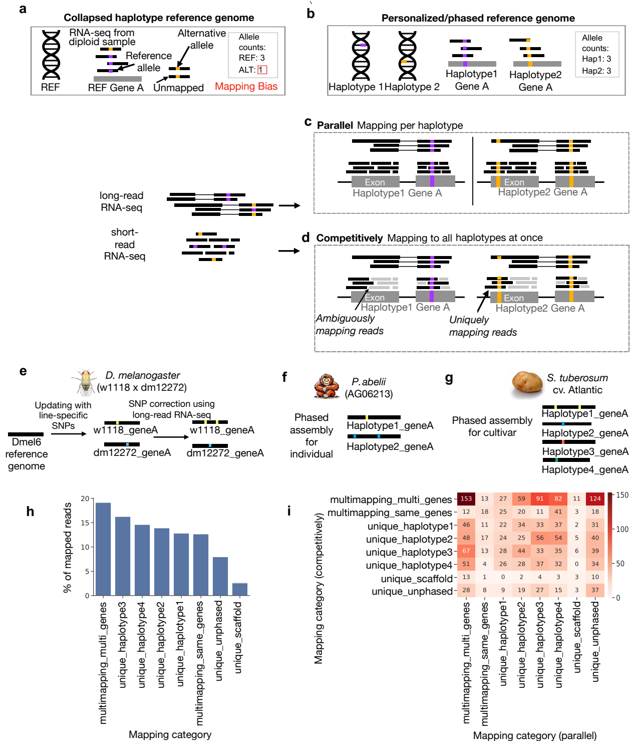
Figure 1: The reference used affects equivalence groups. Tracking multi-mapping results in equivalent allele and genotype counts regardless of the reference used (a) Haploid reference genomes and mapping bias. Reads containing the reference allele may be more likely to align than those containing alternative alleles. (b) Haplotype-phased personalized reference genomes mitigate mapping bias. RNA-seq data
