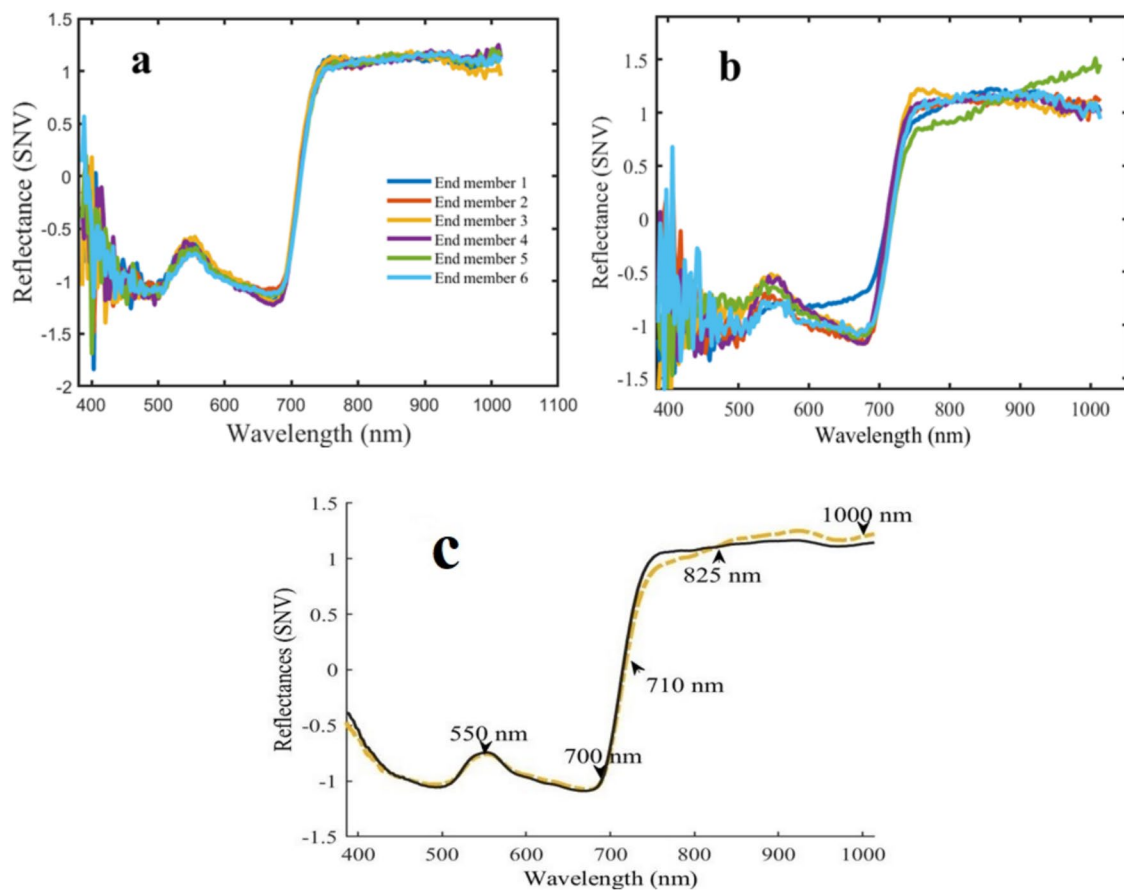
Fig. 5 Six endmembers derived from SNV pre-treated a healthy leaves, b leaves with aphid and c the average spectra's, calculated from healthy and infested endmembers. Three different regions
