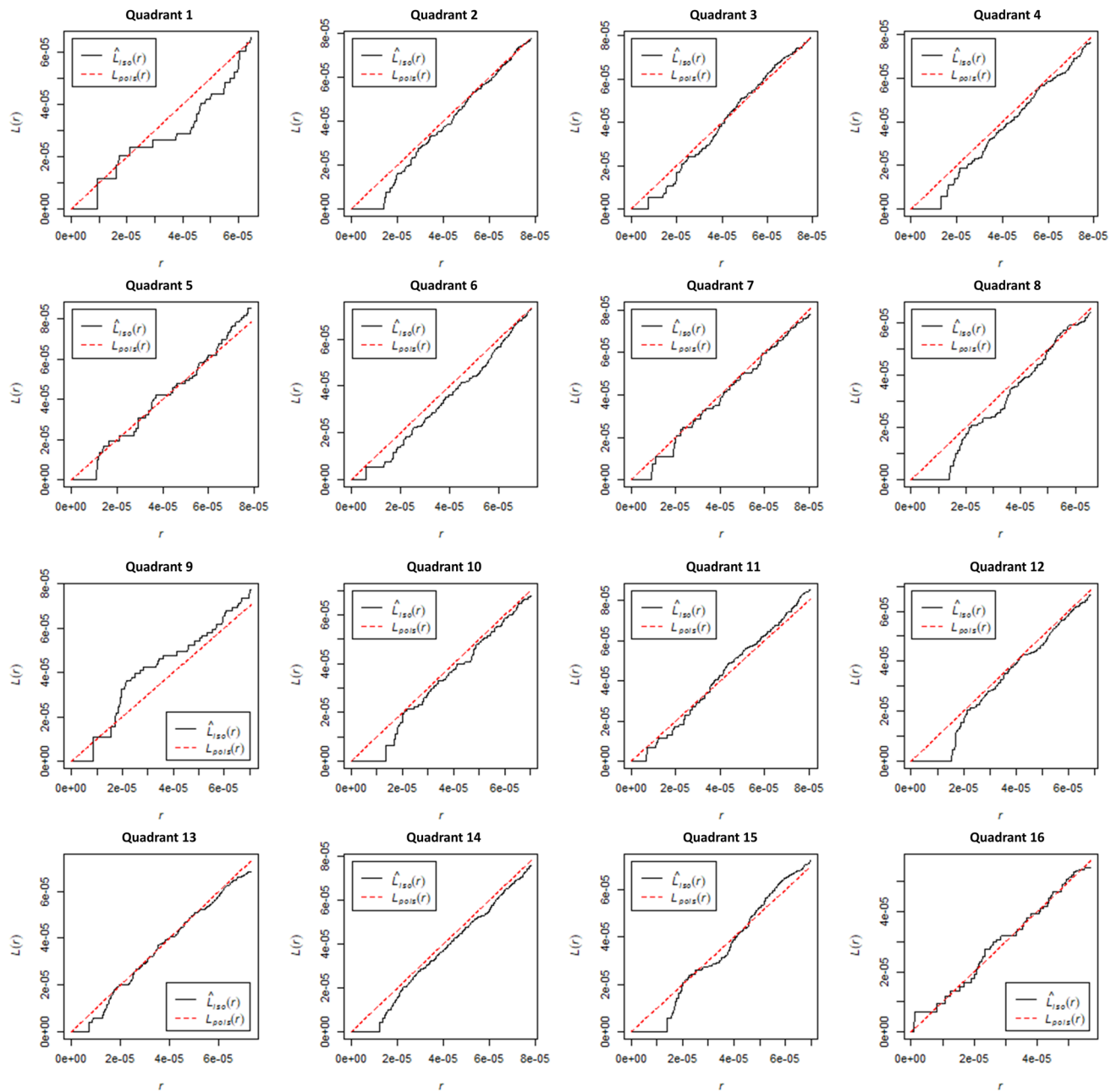
Fig. 7 L – function for all quadrats
