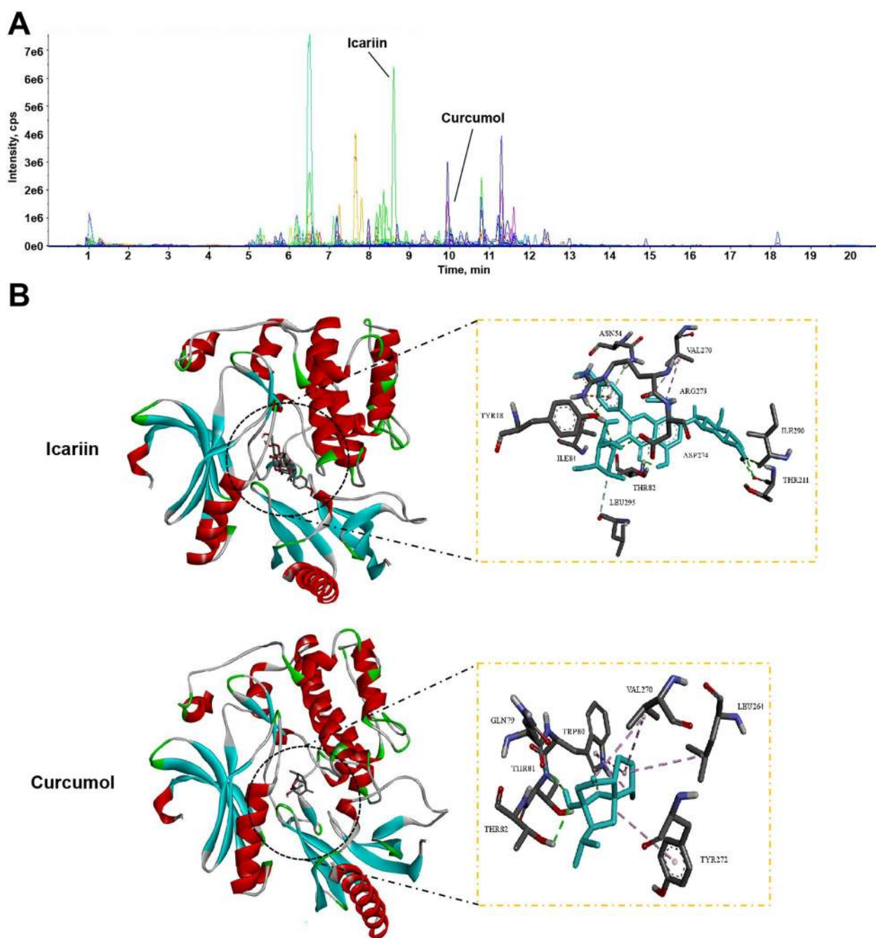
Fig. 4 Icariin and curcuminol can dock with AKT1. (A) The representative LC-MS chromatograms of ECE in negative and positive modes. (B) Molecular docking of icariin or curcuminol and Akt1
