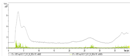
Figure 1: Total Ion Chromatogram (Negative mode) obtained from LC-MS/MS
