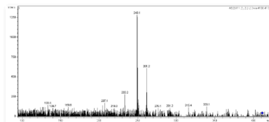
Figure 2: MSMS obtained from LC-MS/MS - (Iso)Pentyl Dihexoside
