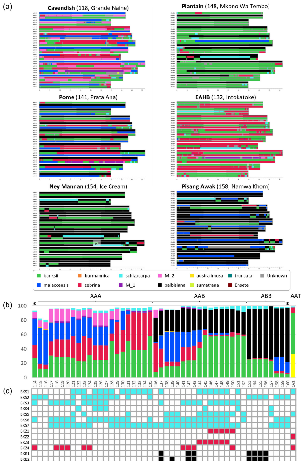
Figure 3. Genome ancestry of triploid banana cultivars. (a) Contrasting genome ancestry mosaics of some popular triploid banana cultivars. Ancestral group contributions are presented along the 11 Musa reference chromosomes by different colors. The representation is based on non-phased genotyping data. Banana subgroups are indicated in bold, accession names are shown in between brackets. Segmental aneuploidy regions are indicated by whitish squares. (b) Cumulative proportions of the genome covered by each ancestry for each triploid cultivar are presented. Main banana genomic groups are indicated on top. A, M. acuminata ; B, M. balbisiana ; T, Australimusa . The color code is described in the above legend. Numbers at the bottom correspond to accessions listed in Table S1. Accessions are mainly triploids, and * indicates tetraploid accessions Calypso (114) and Pisang Awak (160). (c) Results of schizocarpa/banksii (BKS1–BKS7), zebrina/banksii (BKZ1–BKZ4), and banksii/balbisiana (BKB1 and BKB2) breakpoint analysis for polyploid cultivars. Identified breakpoints are shown on the left. Colored squares indicate presence of the corresponding breakpoint.
