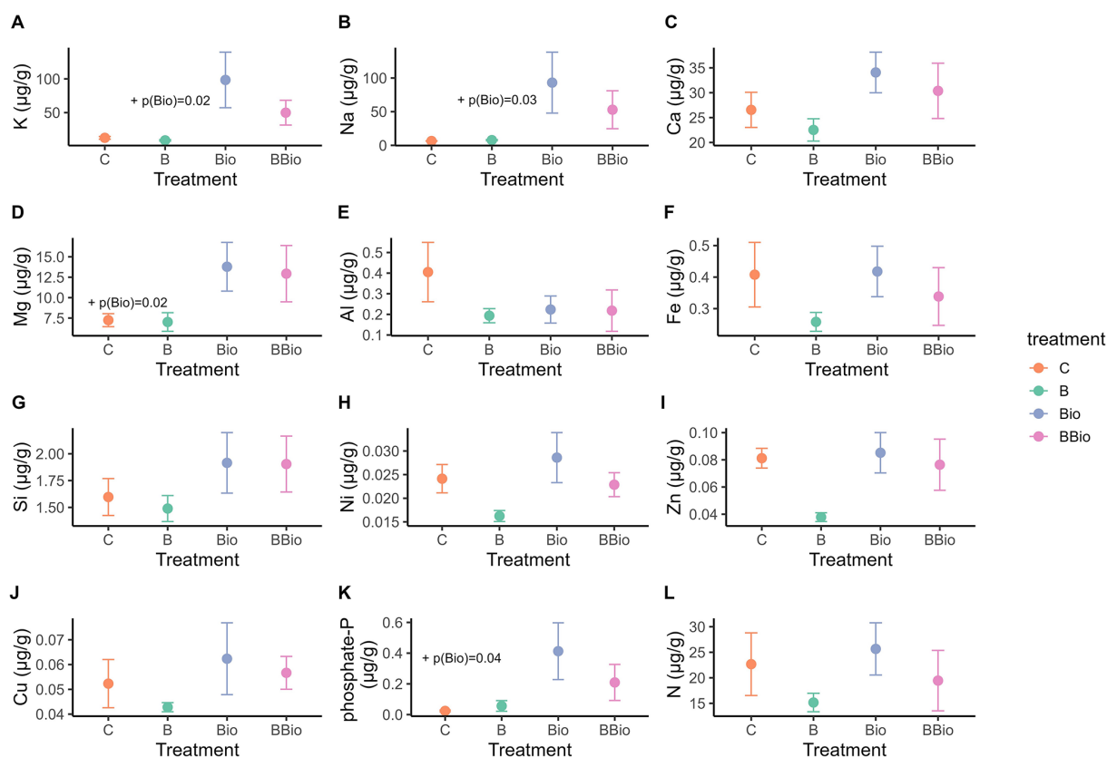
Figure 5. Results from the soil leaching test for samples taken instantly after basalt and biochar amendments. Dots and error bars represent averages and standard errors of the mean. P(B) and p(\text{Bio}) are p values for basalt and biochar, respectively. Significant positive and negative effects are indicated with a + and – respectively.
