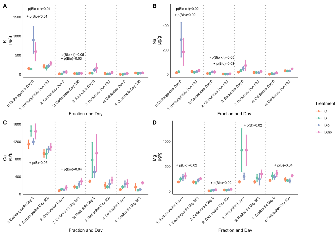
Figure 3. (A) K, (B) Na, (C) Ca and (D) Mg in \mu\text{g element g}^{-1} soil for different soil fractions in clover plots for different sampling times (initial = directly after amendment and last = after 550 d). Dots and error bars represent averages and standard errors. P values for basalt, biochar and time effects ( p(\text{B}) , p(\text{Bio}) , p(t) respectively) are annotated on the plots. Significant positive and negative effects are indicated with a + and – respectively. A vertical dotted line is plotted in between different soil fractions.
