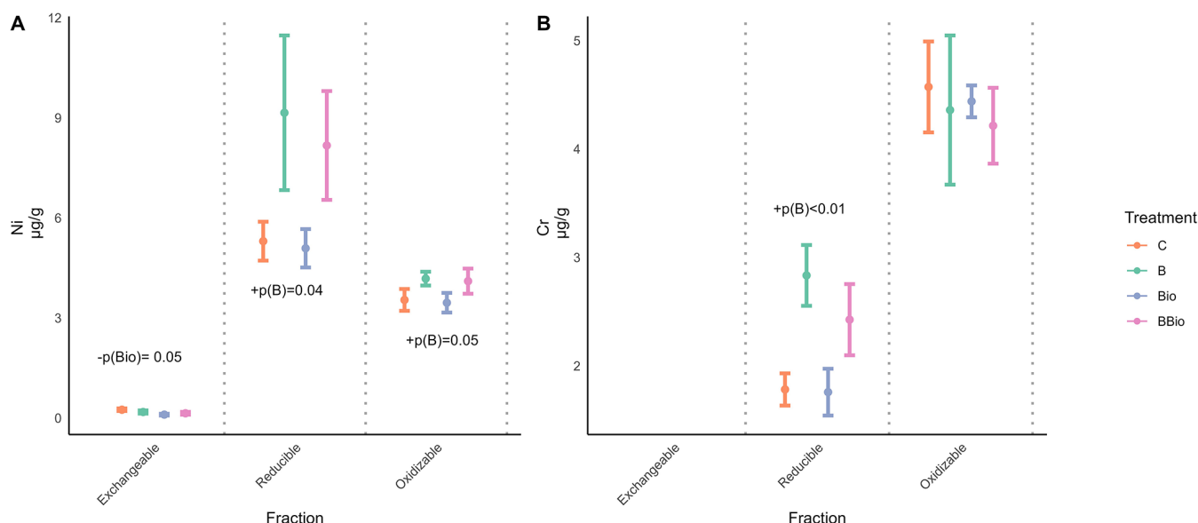
Figure 4. Ni and Cr in the 4 different considered soil fractions. These soil elements were extracted after initial soil sampling in clover plots. P(B) and p(\text{Bio}) are p values for basalt and biochar, respectively. Carbonate-Ni, carbonate-Cr and exchangeable Cr were below detection limits and are not shown in this plot. Significant positive and negative effects are indicated with a + and – respectively. A vertical dotted line is plotted in between different soil fractions.
