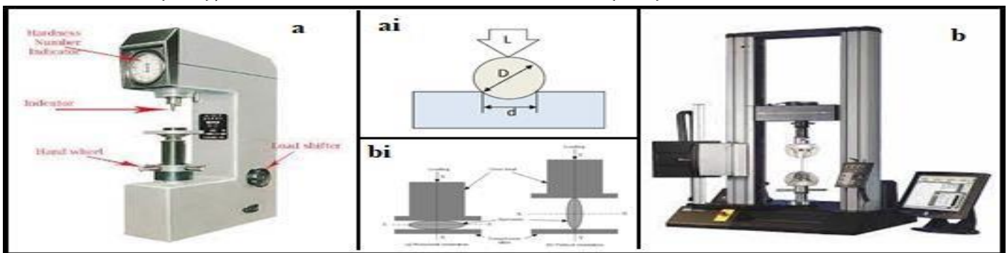
Figure 2. The Brinell Hardness Tester is shown in (a) and the test demonstration (ai).
