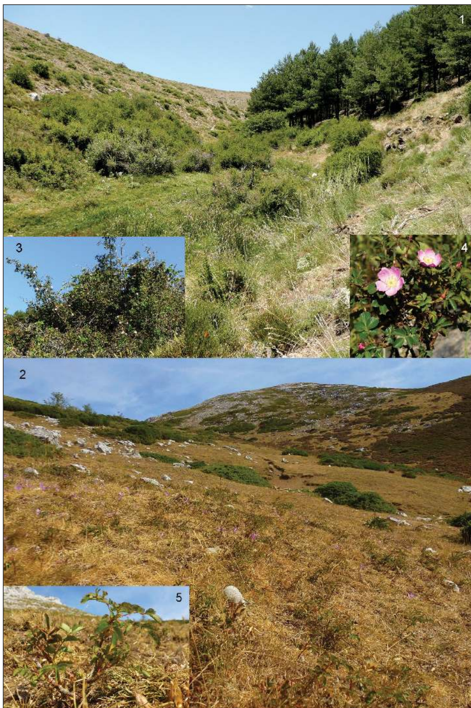
Figures 1–5. Habitats and foodplants of Spialia rosae in the Iberian Peninsula. 1. Habitat in Puerto de la Ragua, 2090 m (Sierra Nevada, Spain, July 2011). 2. Habitat in Pico Yordas, 1700 m (Cantabrian Mountains, Spain, September 2012). 3. Plant of Rosa sicula (July 2013). 4. Flowers of R. sicula (July 2013). 5. Plant of R. pendulina (September 2012).
