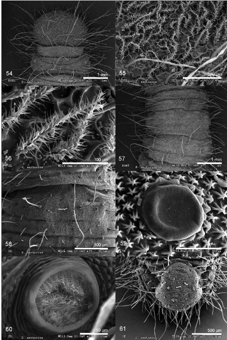
Figures 54–61. Scanning electron microscope images of a last instar larva of Spialia sertorius from Losar de la Vera, Cáceres, Central Spain. 54. Head capsule and collar. 55, 56. Detail of the head capsule setae and sculpture. 57. Cuticular formations on thoracic and abdominal segments. 58. Detail with different types of subdorsal and lateral setae on the first thoracic segment: long and short setae with pointed tips. 59. Detail of a barrel-like formation and the cuticular sculpture. 60 Last abdominal spiracle. 61. Last abdominal segments with the anal plate and setae with pointed tips and rounded bases.
